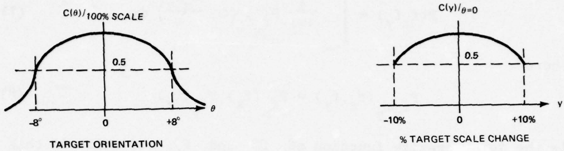
Fig. 11 Variation of Correlation Signal C with Target Parameter Changes Such as Orientation and Scale
