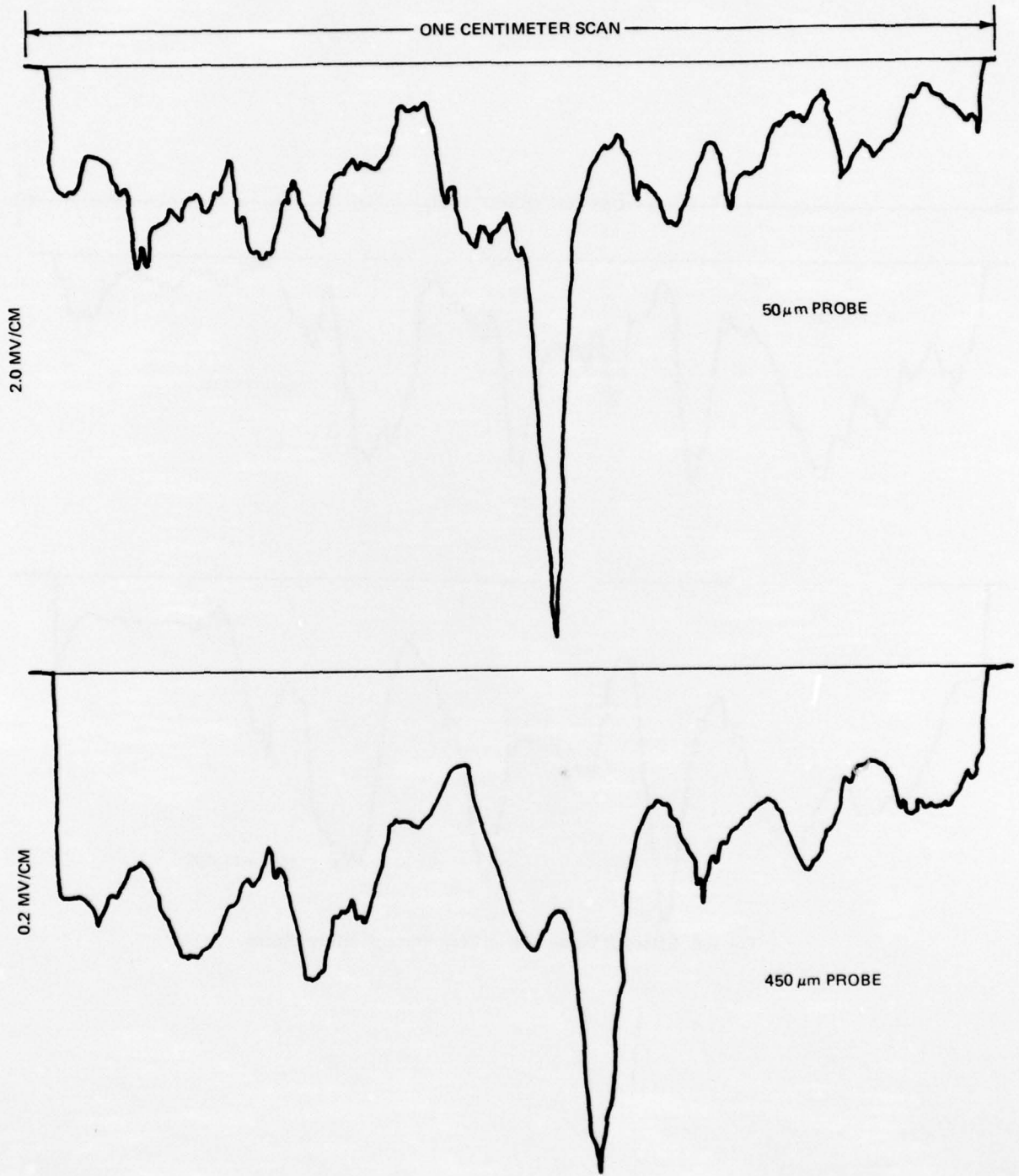
Fig. A-4 Effect of Probe Size on Scan Through M-60 Tank in River/Island Scene
