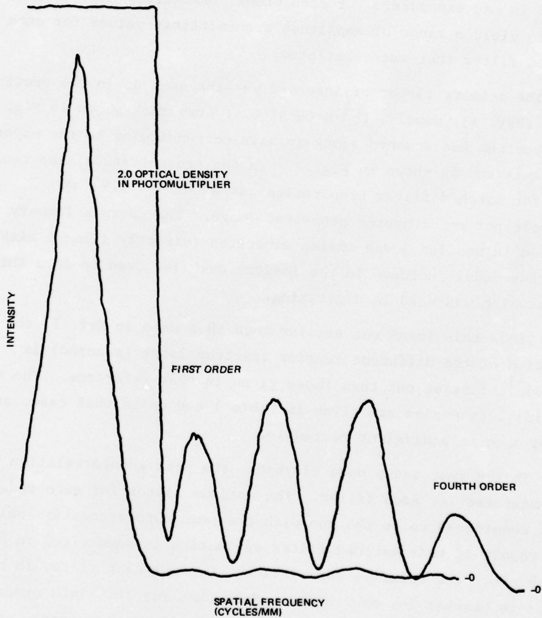
Fig. 2 M-60 Spectrum Scan Perpendicular to Major Axis (Parameters: 450 \mu\text{m} Probe; 4.39 \frac{\text{cycles}}{\text{mm}} /mm Scale Sensitivity; 360mm Focal Length)
