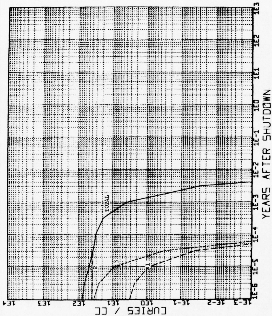
Fig. B-4 Radioactive Decay Curves for P
