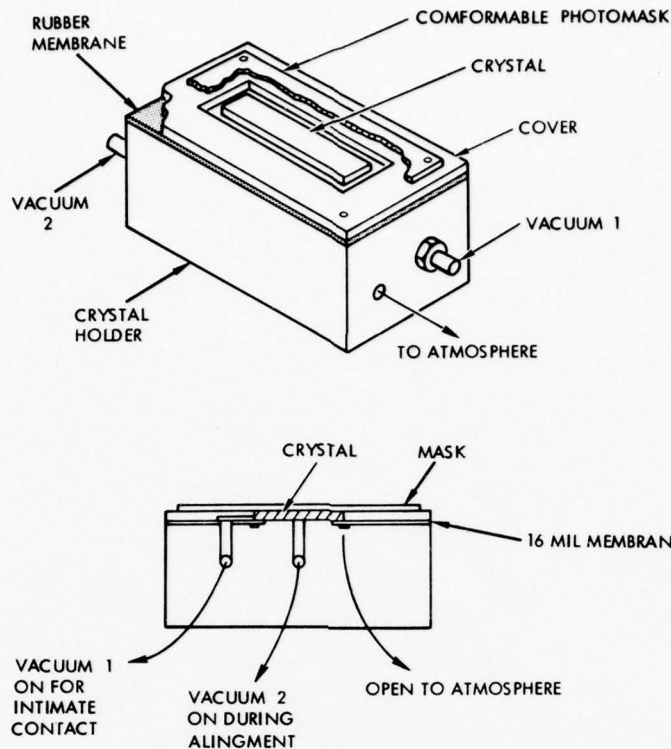
Figure 2-8. Vacuum Frame Operational Details
