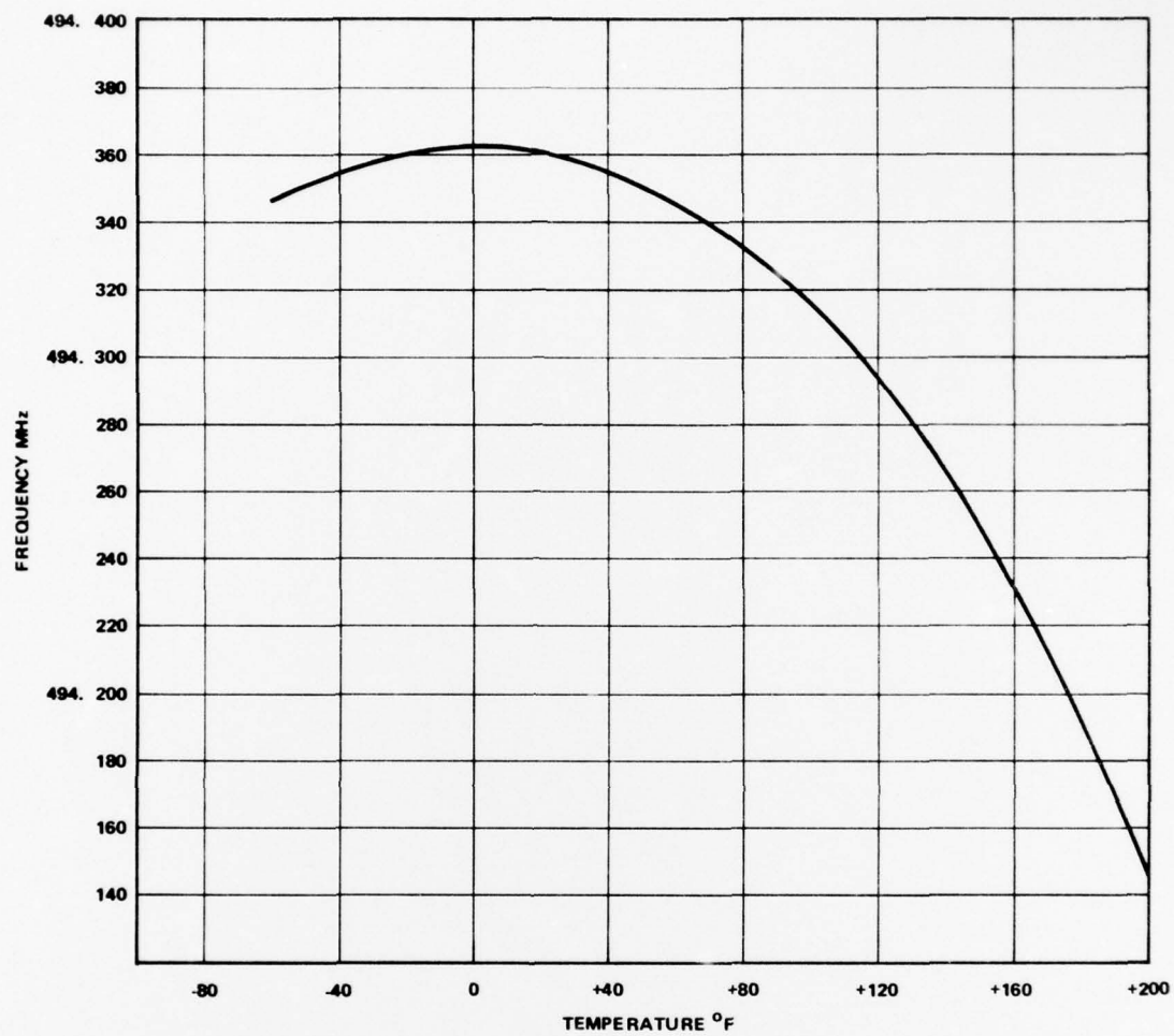
Figure 4-26. 500 MHz SAW Output Frequency as a Function of Baseplate Temperature
