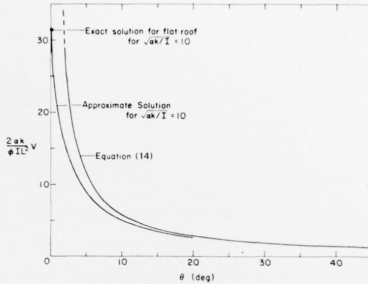
Figure 5. Dimensionless volume of water in the saturated layer [(2\alpha k_s / \phi IL^2)V] shown for given parameters as a function of roof slope. The solution for V given by eq 14 is only approximate and as the roof slope decreases, the error increases. Accordingly an approximation to the solution is given for small values of \theta .
