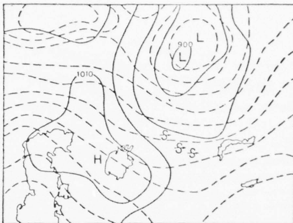
Figure 5. Dust storms in a high cyclone at Bet Pak Dala, Dzhetikonur, and Karsakpay stations, 1500 hours, 4 August 1957.
