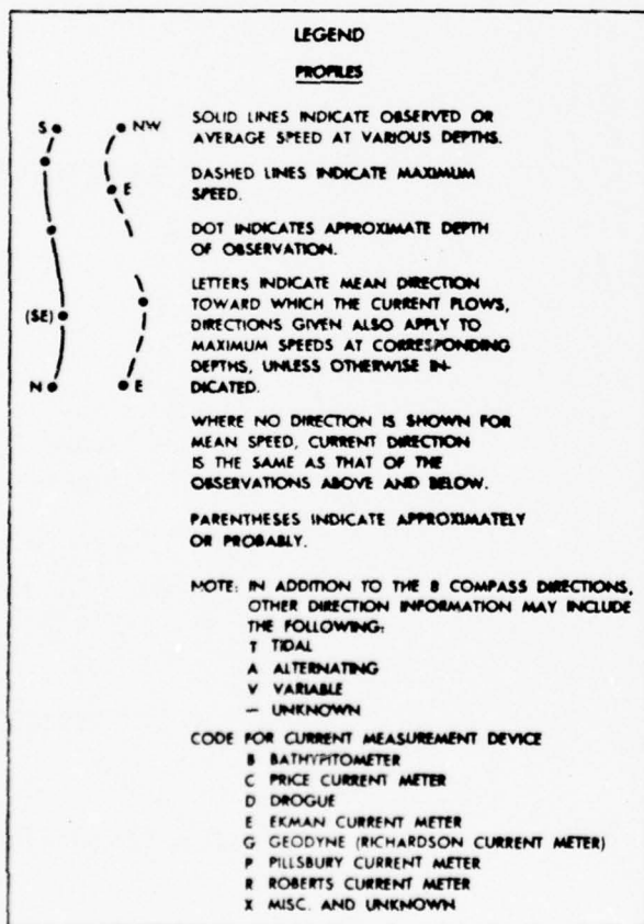
Figure 12. Subsurface Currents In The Tongue Of The Ocean (Northern Portion) ref.2
