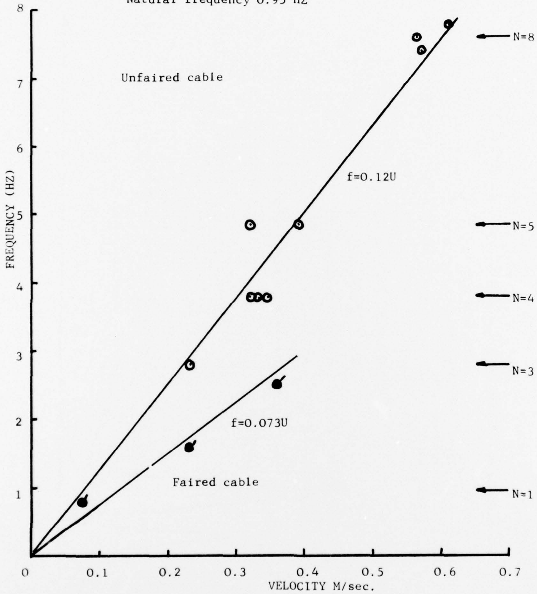
Figure 24. Effect Of Anti-Strumming Fairing On Frequency
