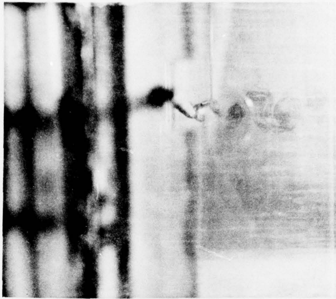
a. Vortex Shedding from Bare Tubing
