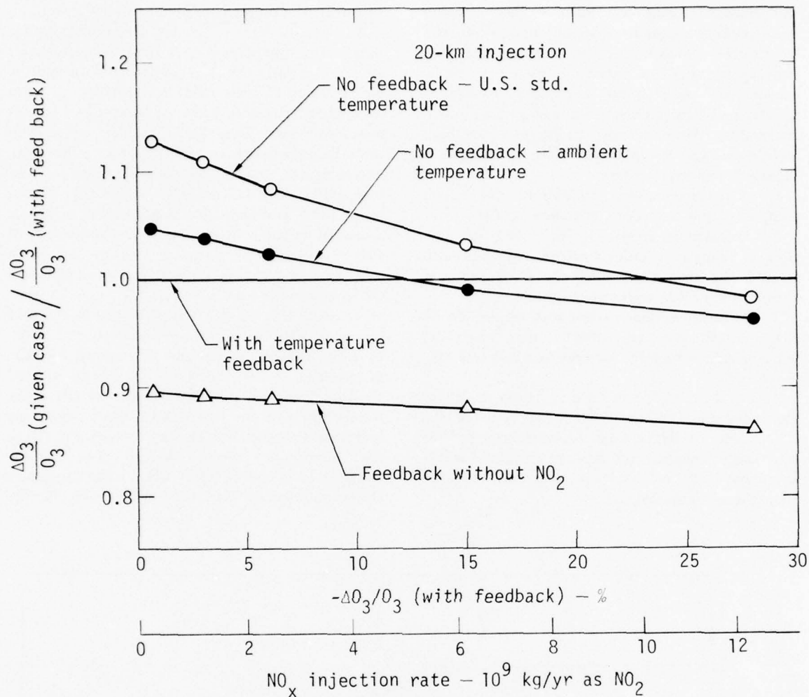
Fig. 25. Calculated ratio of ozone reduction for a given case to ozone reduction with feedback vs \text{NO}_x injection rate for a 20-km injection height.
