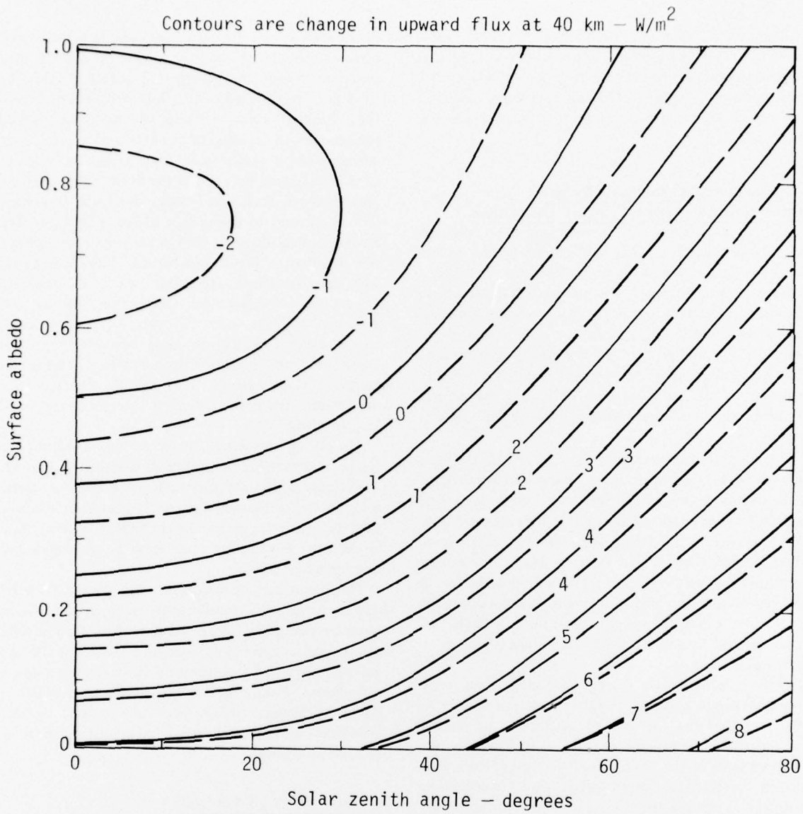
Fig. 30. Calculated change in upward flux at 40-km altitude as a function of surface albedo and solar zenith angle. Solid curves are full-flux calculation, dashed curves are one-wavelength (0.55- \mu m ) calculation.
