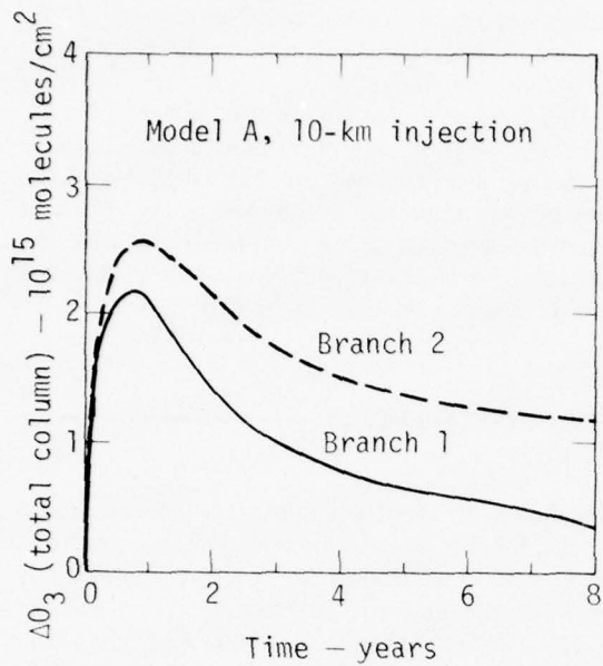
Fig. 17. Calculated change in the total O_3 column vs time as a result of an NO_x injection (as NO_x ) of 2000 molecules/cm 3 ·s in a 1-km-thick layer centered at 10 km.
