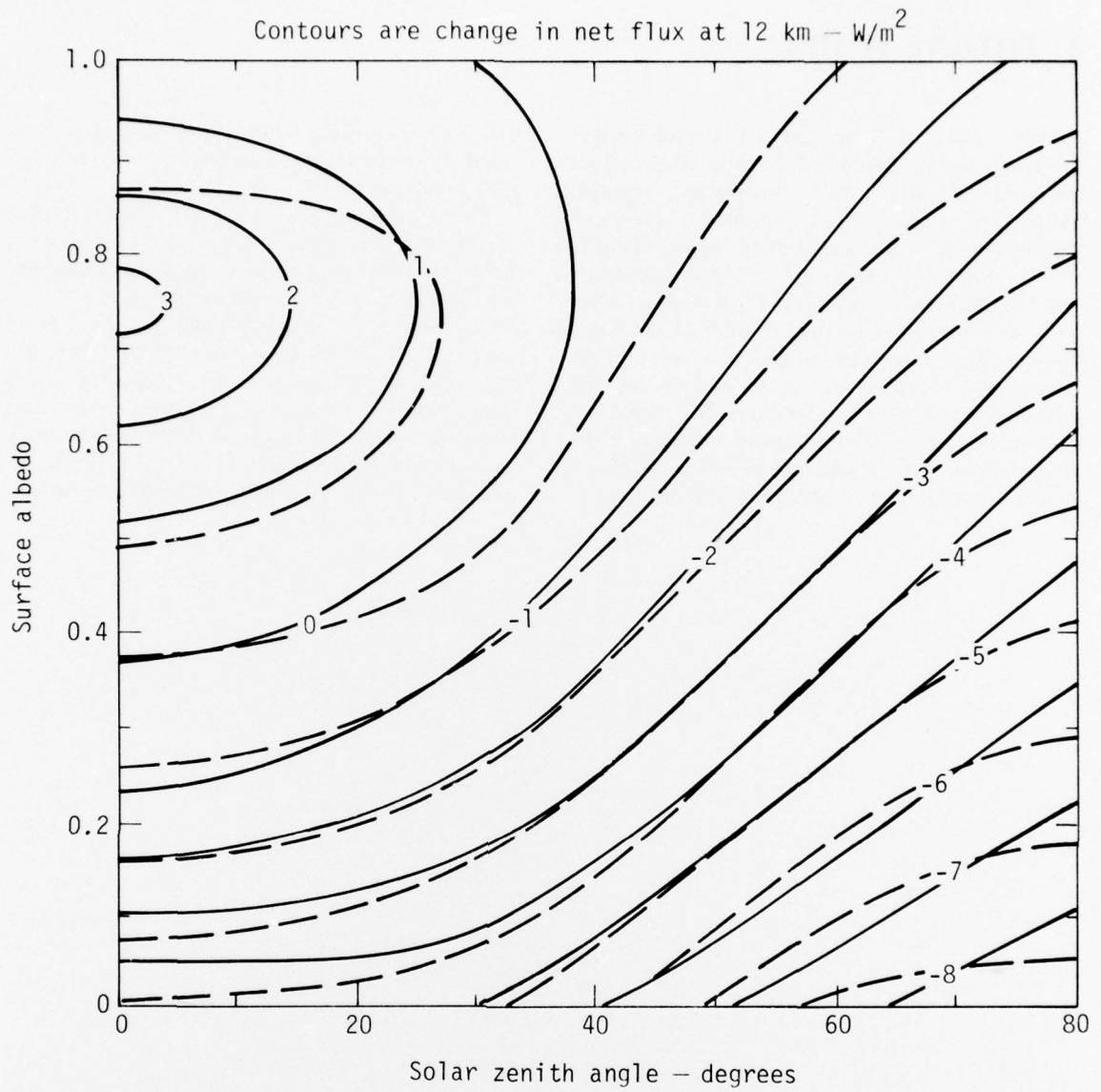
Fig. 31. Calculated change in net flux at 12-km altitude as a function of surface albedo and solar zenith angle. Solid curves are full-flux calculation, dashed curves are one-wavelength ( 0.55\text{-}\mu\text{m} ) calculation.
