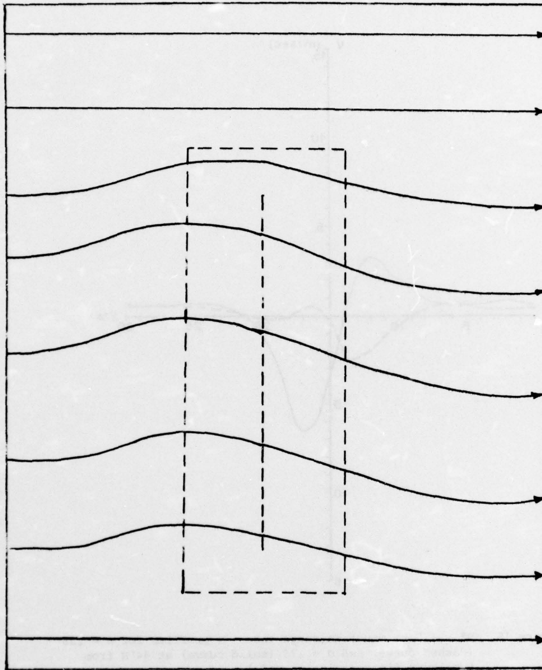
Figure 17. 9° x 1.5 km mountain range case. Six-layer coarse resolution model streamlines for \sigma = .75 .
