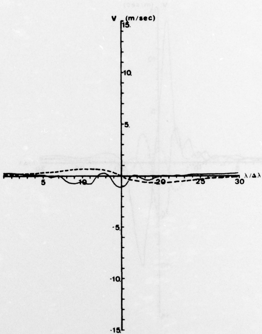
Figure 23. 3^\circ \times 1.5 km mountain range case. Analytic v-profile for \sigma = 0 (dashed curve) vs. six-layer fine resolution model profile for \sigma = .08333 (solid curve). Both at 44^\circ\text{N} .
