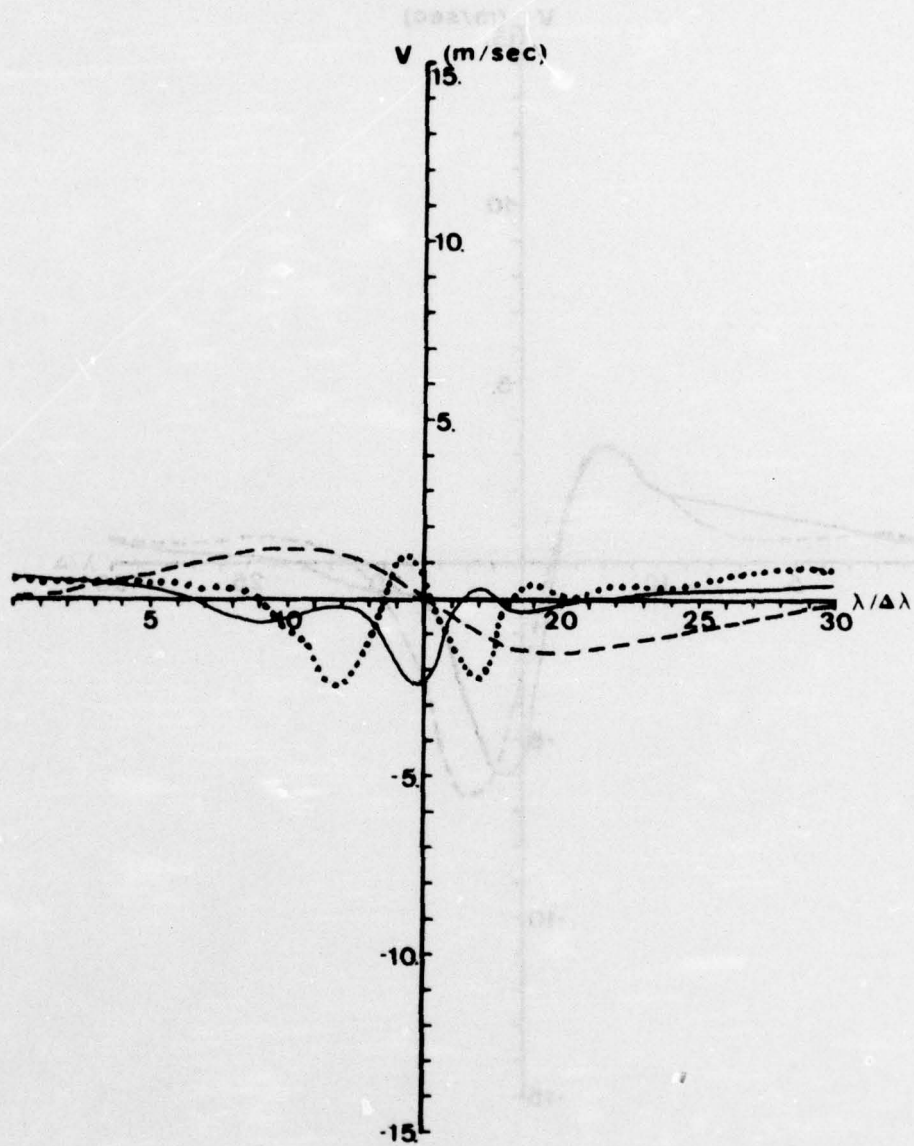
Figure 14. 9^\circ \times 1.5 km mountain range case. Analytic v profile for \sigma = 0.0 (dashed curve) vs. six-layer fine-resolution model v profiles for \sigma = .083333 (solid curve) and \sigma = .25 (dotted curve), all at 44^\circ\text{N} .
