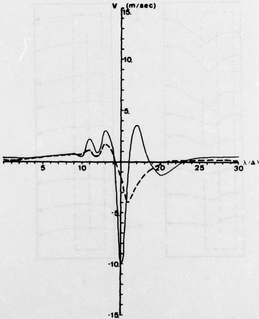
Figure 25. 3^\circ \times 1.5 km mountain range case. v-profiles for \sigma = .75 at 44^\circ\text{N} from six-layer fine resolution model (solid curve) and two-layer fine resolution model (dashed curve).
