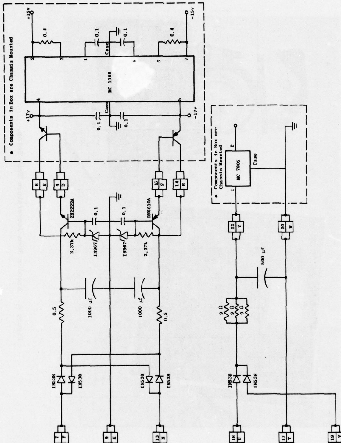
Figure 7. Magnetic Shaft Encoder Power Supply.
