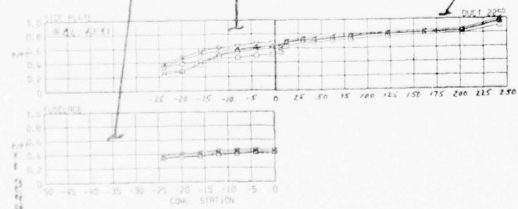
Flow field versus angle of attack ( \beta = 0^\circ ) for the Basic Inlet-Plate Inlet at W_c = 310 pps.
