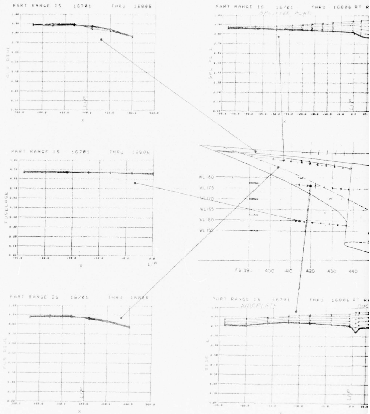
Figure 28. M_0 = 0.5 inlet-flow-field data for the B Inlet at B.L. 43.82 at \alpha = 2^\circ and \beta = 0
