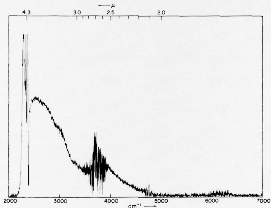
Figure 3. \text{CO}_2 Hot Cell Spectrum: Resolution 1.9\text{ cm}^{-1} , Gas Temperature 625^\circ\text{K} , Raw Spectrum
