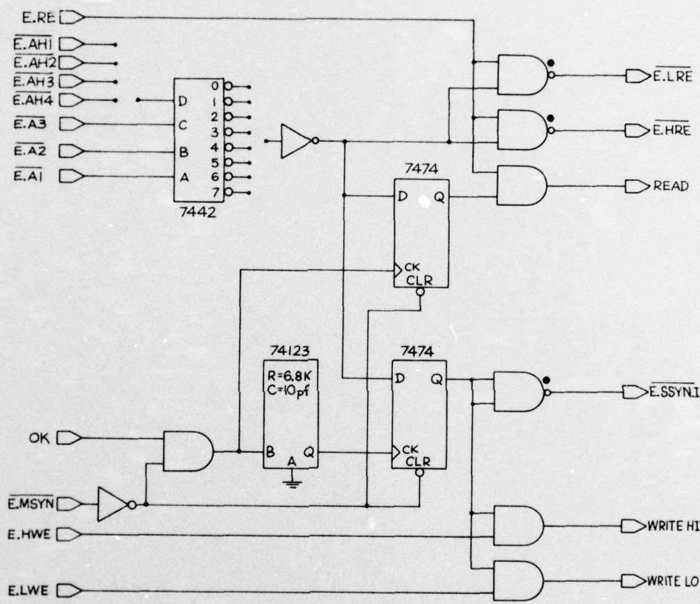
ADDRESS DECODER
