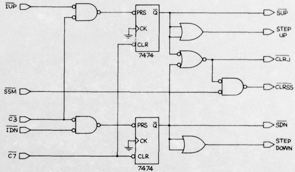
STEP GENERATOR
