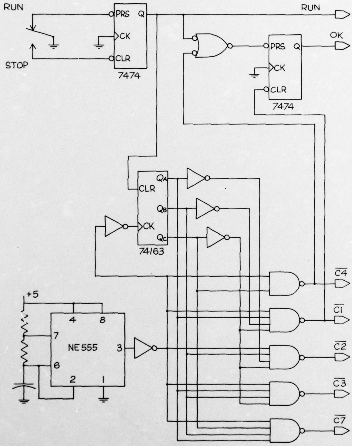
MULTI-PHASE CLOCK
