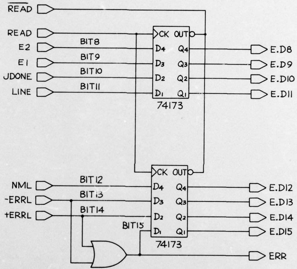
STATUS REGISTER- BITS 8-15
