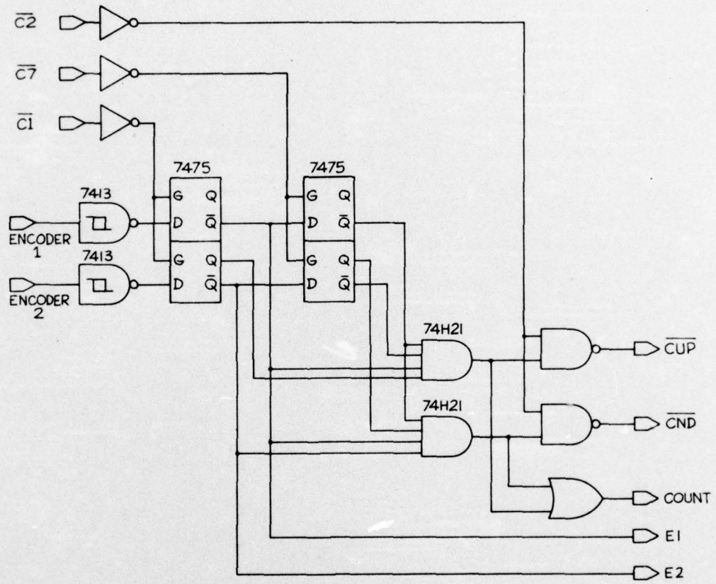
SHAFT-ENCODER DECODER
