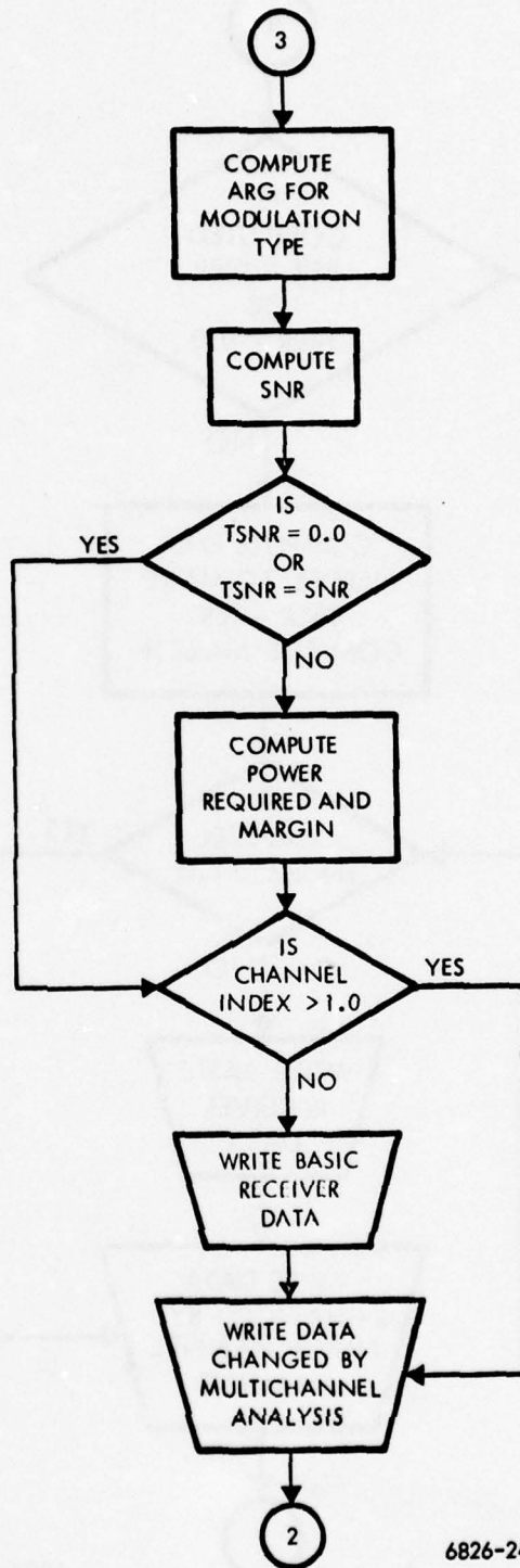
Logic Diagram for RAM (Sheet 4 of 4)
