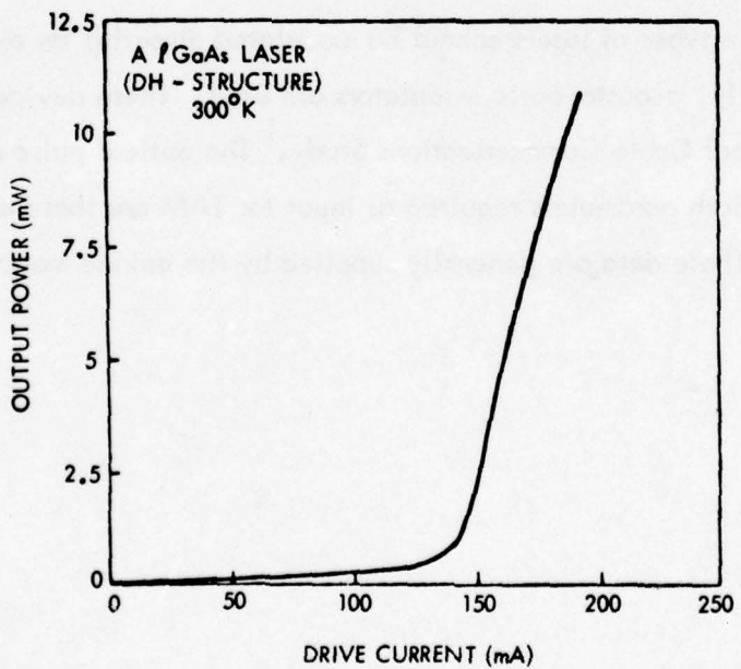
Figure 2.4.3.3-1. ILD and LED L-I Characteristics
