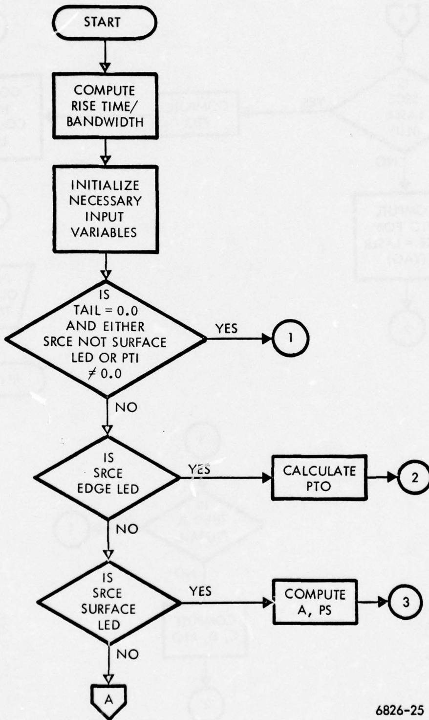
Logic Diagram for TAM (Sheet 1 of 2)
