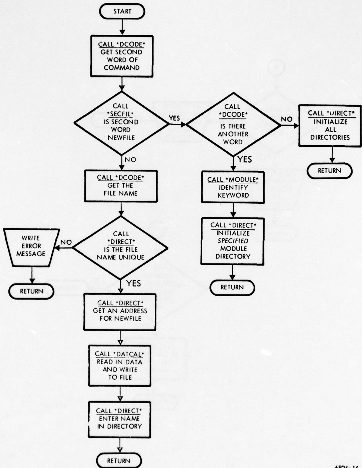
Logic Diagram for CREATE
