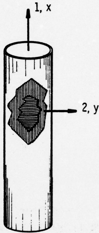
[0/90]_s LAYUP
