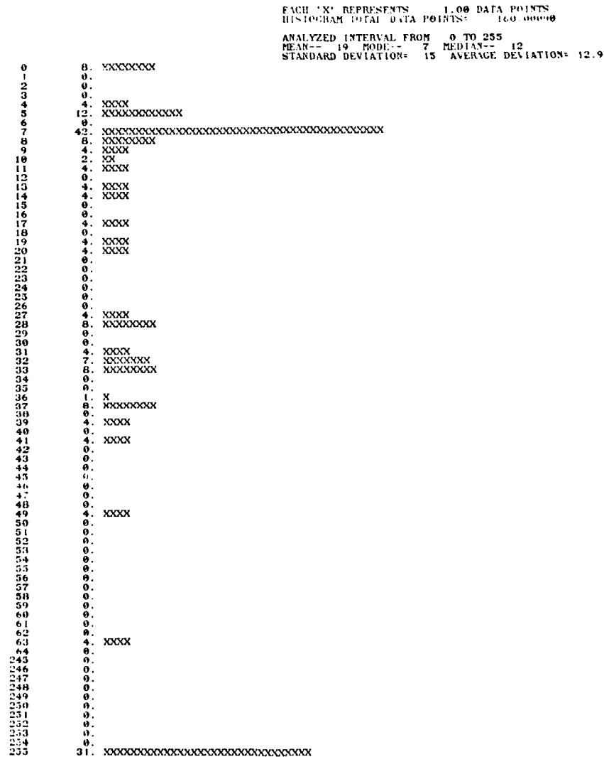
Figure 13. Histogram of cursor located field around man-made object in scene (car).
