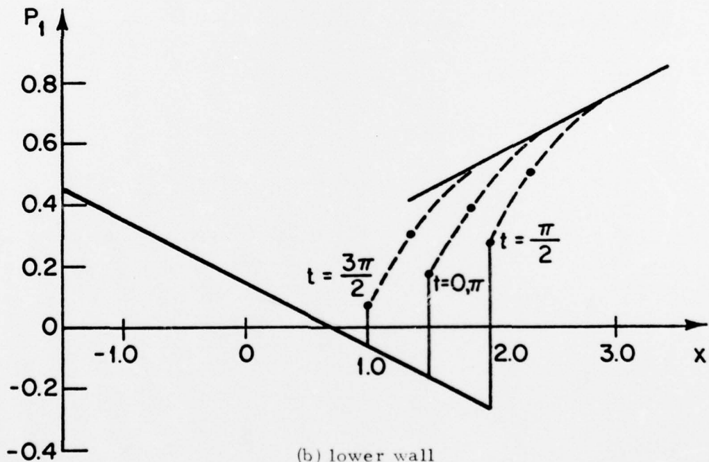
Figure 8. First order wall pressure distributions for various times for channel walls given by equation (43) and shock location as in equation (44). \gamma = 1.4 , \epsilon = 0.1 . — calculated pressure distribution upstream of the shock wave, jump across shock, and outer pressure distribution downstream of shock. ● pressures calculated in inner region. --- approximate pressure distribution in inner region.
