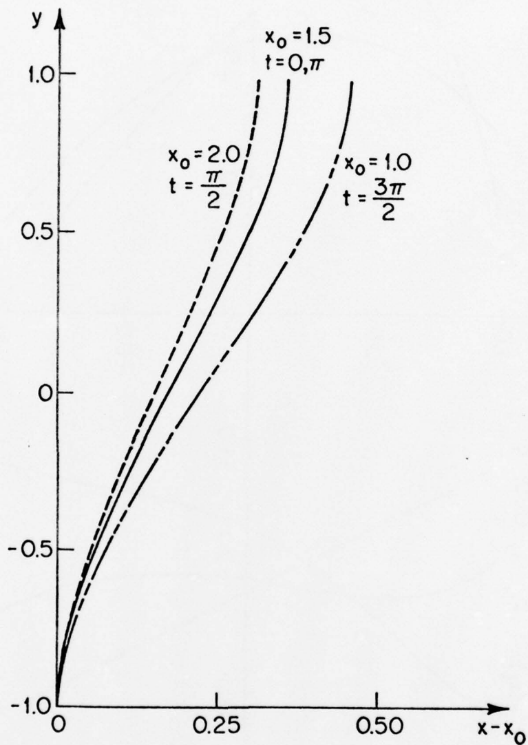
Figure 7. Variation of shock wave shape with time for channel walls given by equation (43) and shock location as in equation (44). \gamma = 1.4 , \epsilon = 0.1 .
