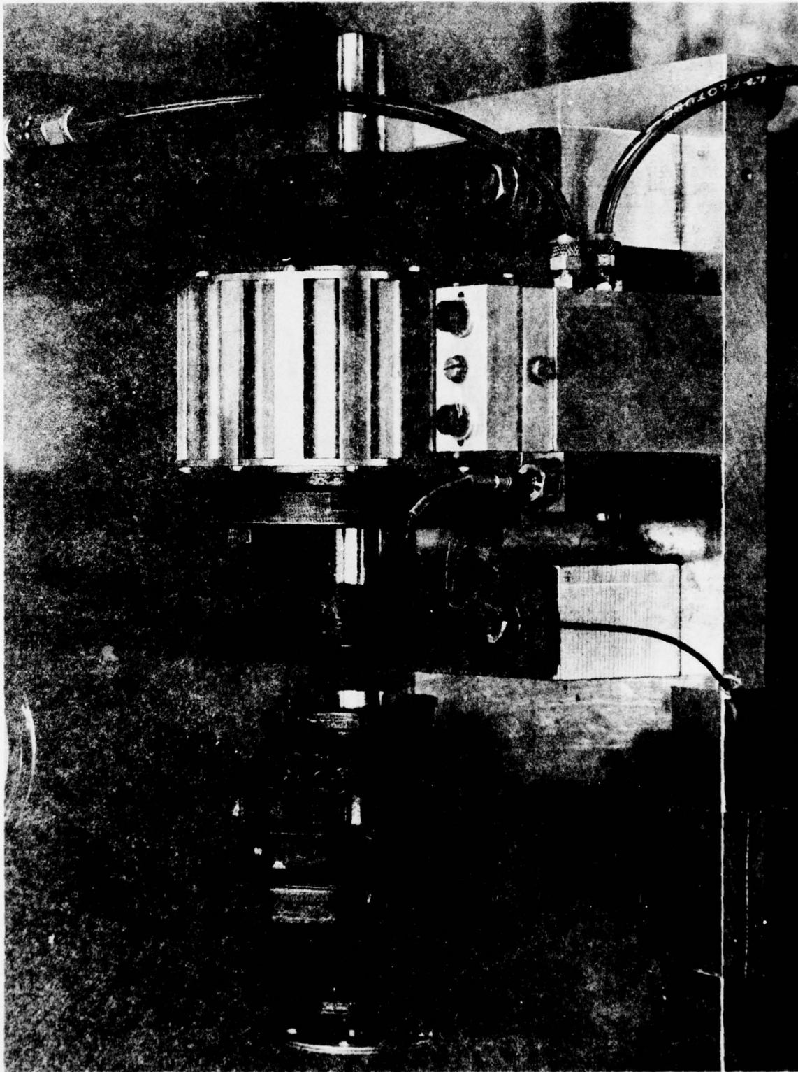
FIGURE 2-2 CHOPPER
