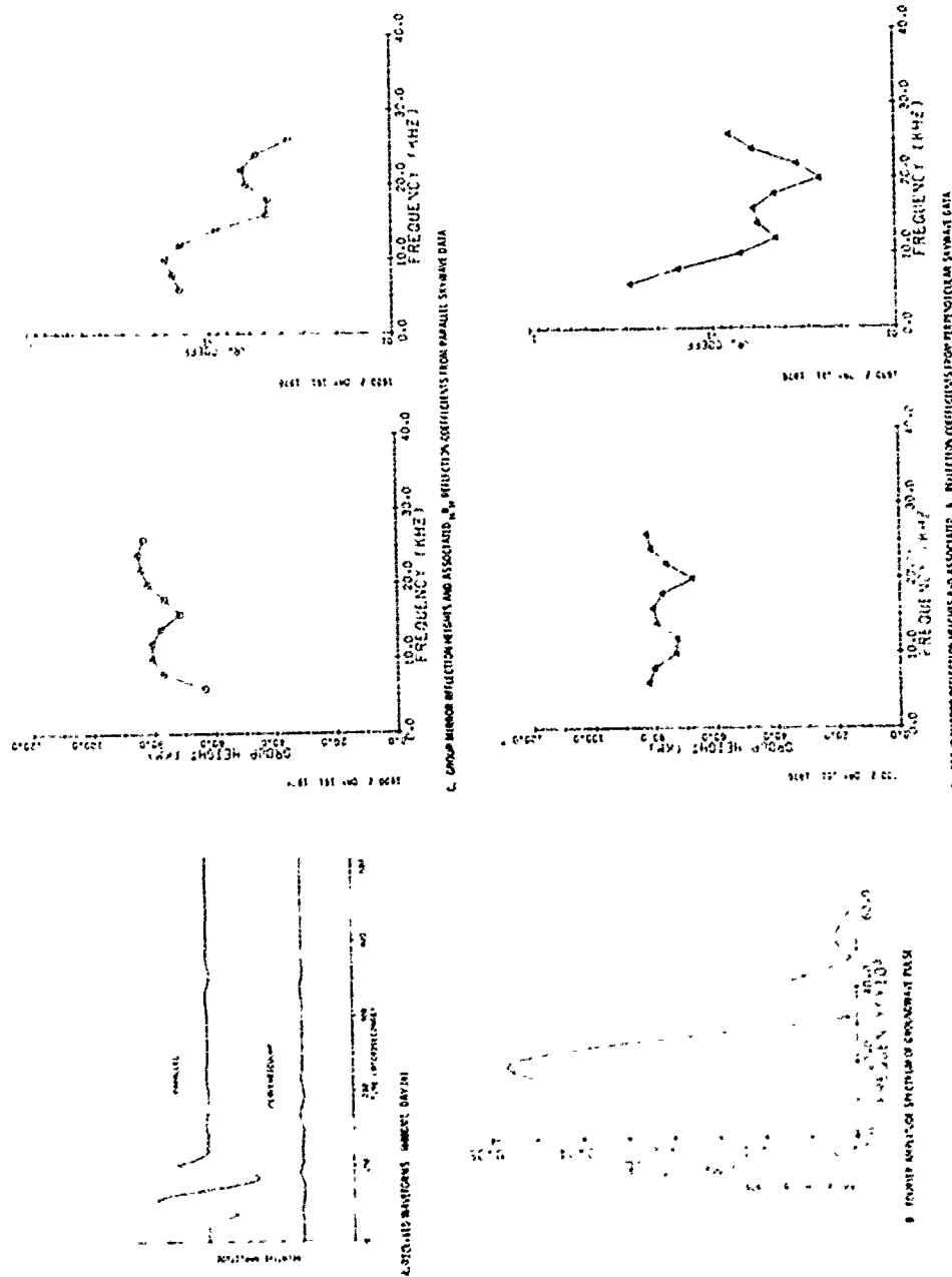
Figure 25. VLF/LF Reflectivity and Ionospheric Data for the Polar Ionosphere, DAY 158 (6 Jun) - DAY 164 (12 Jun) 1976
