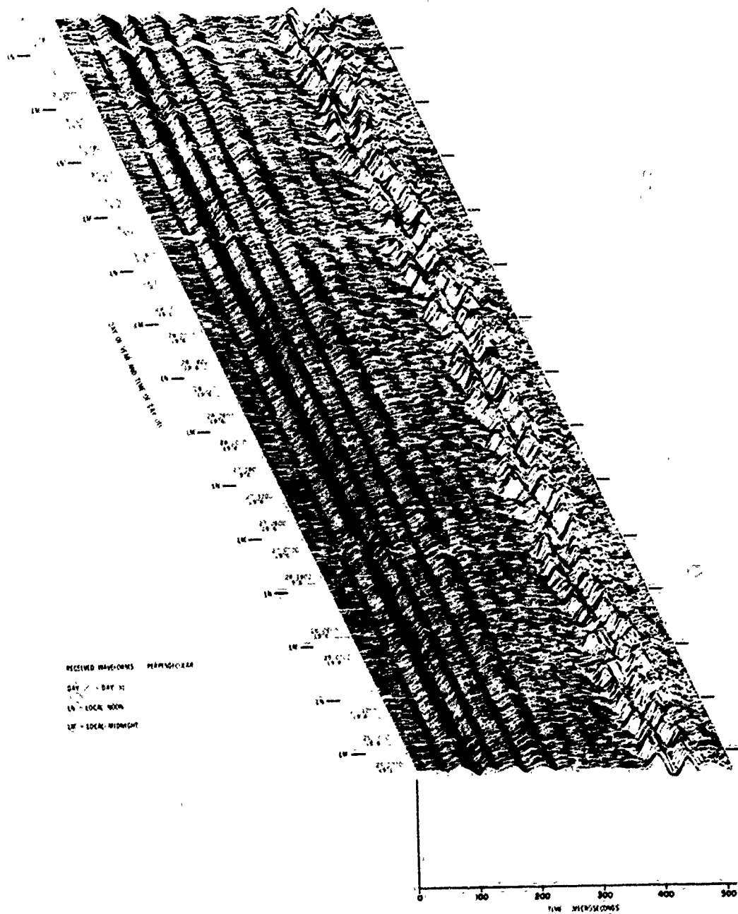
Figure 6. VLF/LF Reflectivity Data for the Polar Ionosphere, DAY 25 (25 Jan) - DAY 31 (31 Jan) 1976 (Cont) Part S. 1 Waveform Display
