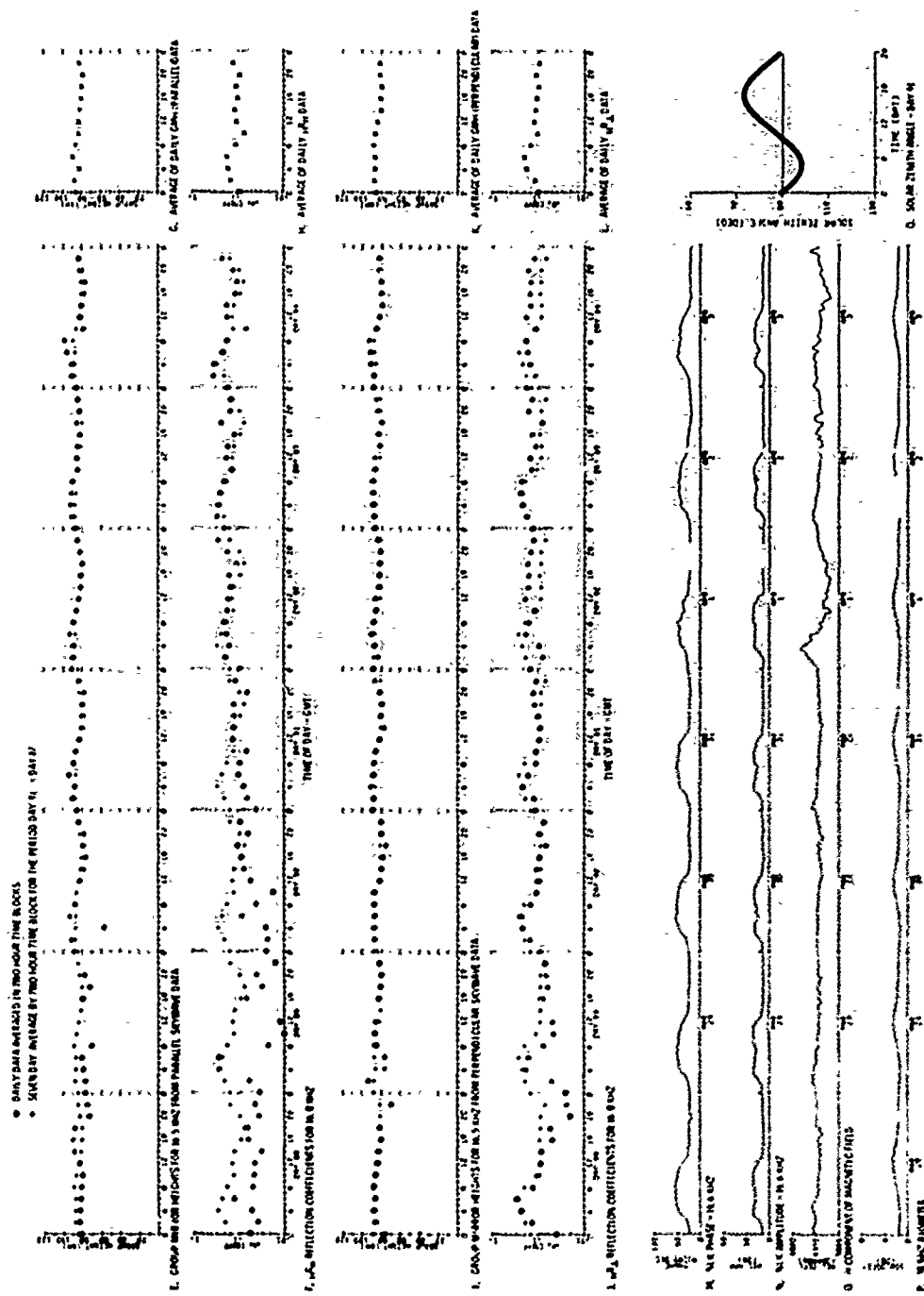
Figure 15. VLF/LF Reflectivity Data for the Polar Ionosphere. DAY 88 (28 Mar) - DAY 94 (3 Apr) 1976 (Cont)
