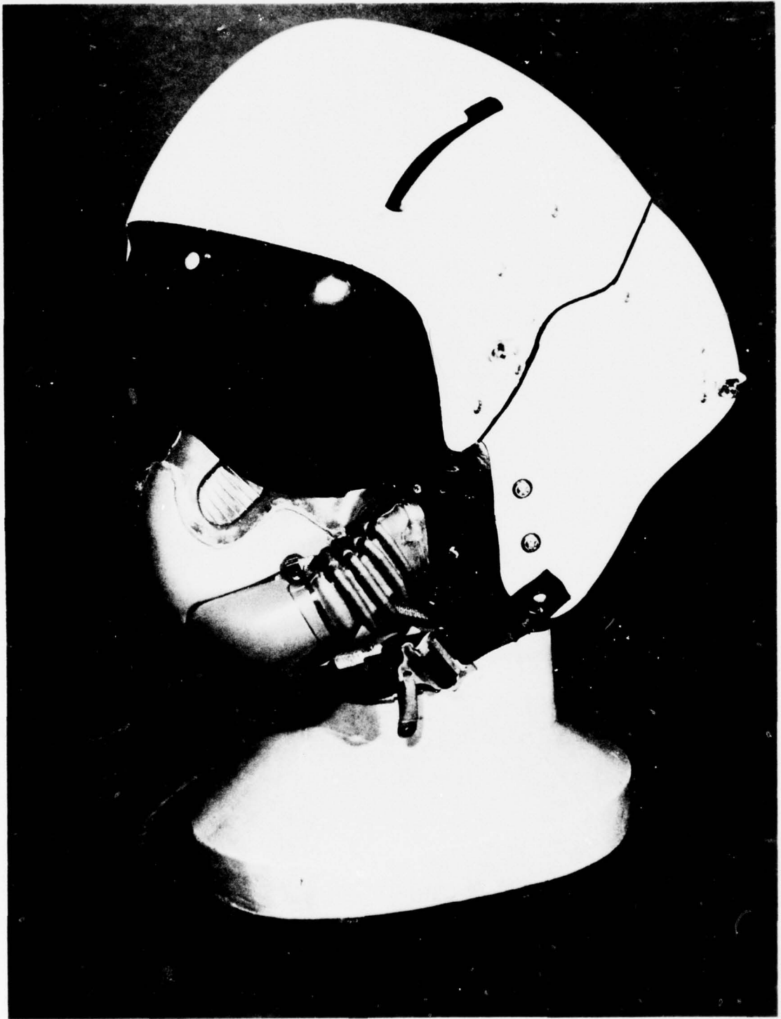
Figure 5. VTAS-III Helmet.
