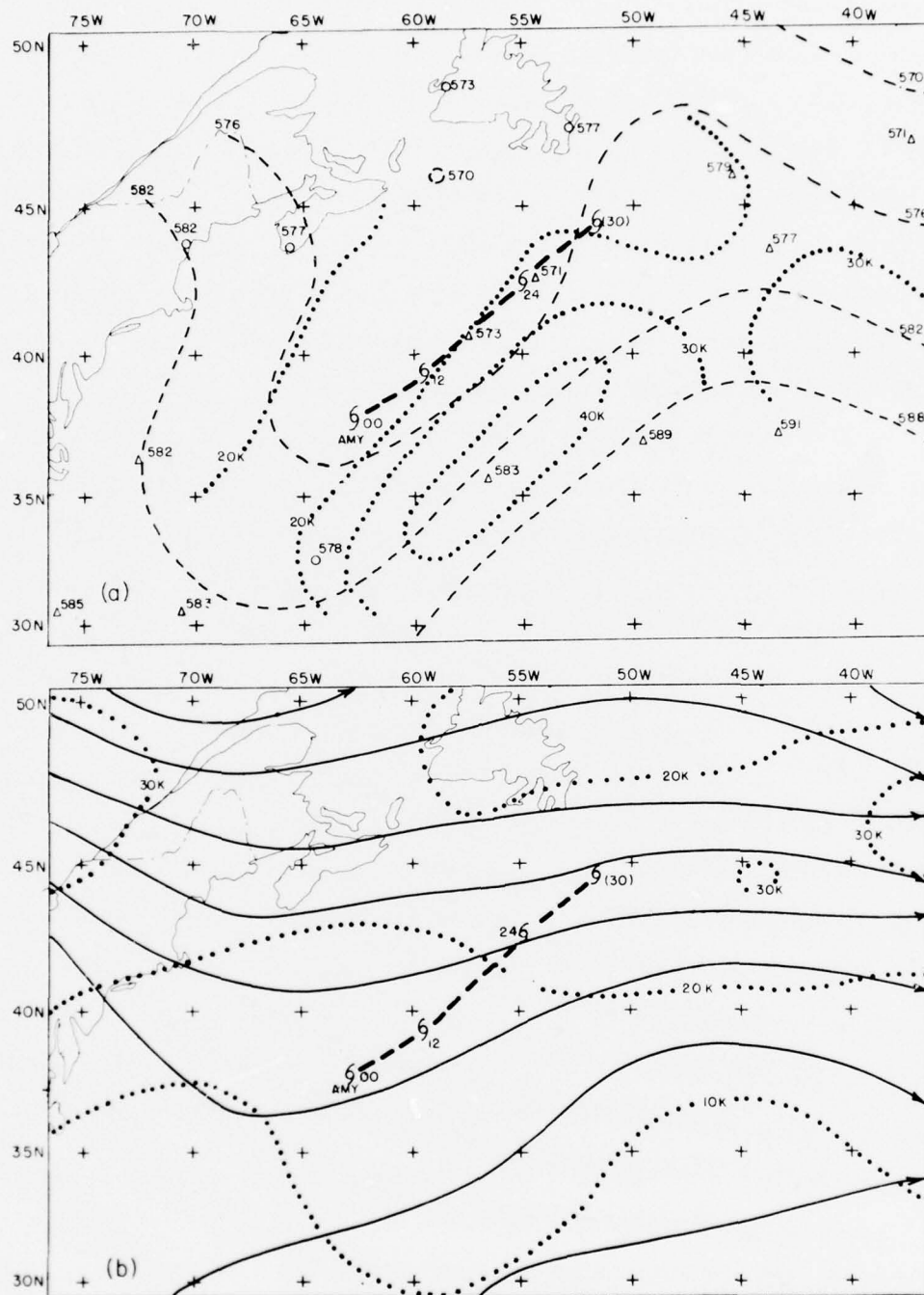
Figure 8. Wind fields from a) the subjective 500-mb geostrophic analysis and b) subjectively-smoothed SANBAR initial analysis. Dotted lines indicate isotachs at 10-kt intervals. Other notation the same as Figure 6.
