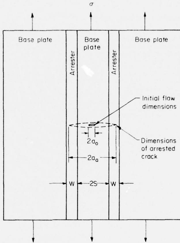
FIGURE 5.1.1. SCHEMATIC REPRESENTATION OF A LARGE, UNIFORMLY STRESSED PLATE WITH TWO WELDED-IN, IN-PLANE, CRACK ARRESTERS OF THE SAME THICKNESS AS THE BASE PLATE
