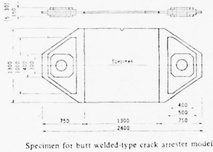
Specimen for butt welded-type crack arrester model
