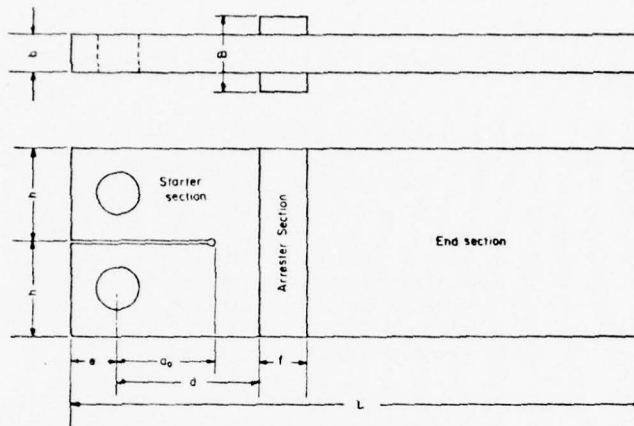
FIGURE 3.6.2. DCB SPECIMEN GEOMETRY FOR ARRESTER CALCULATIONS
