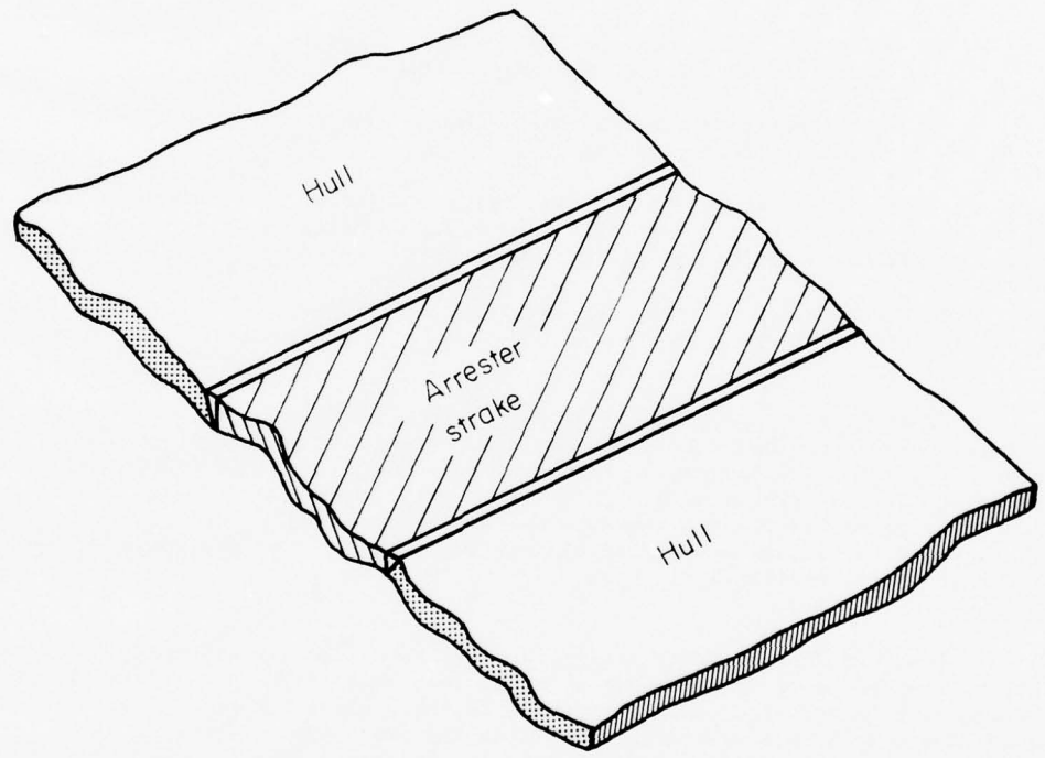
FIGURE 2.2.2. INSERTED TYPE OF CRACK ARRESTER
