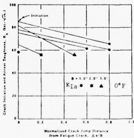
FIGURE 3.3.1. INFLUENCE OF THE CRACK JUMP DISTANCE ON THE ARREST TOUGHNESS, K_{Ia} , OF A533B STEEL AFTER CROSLY AND RIPLING 41 .
