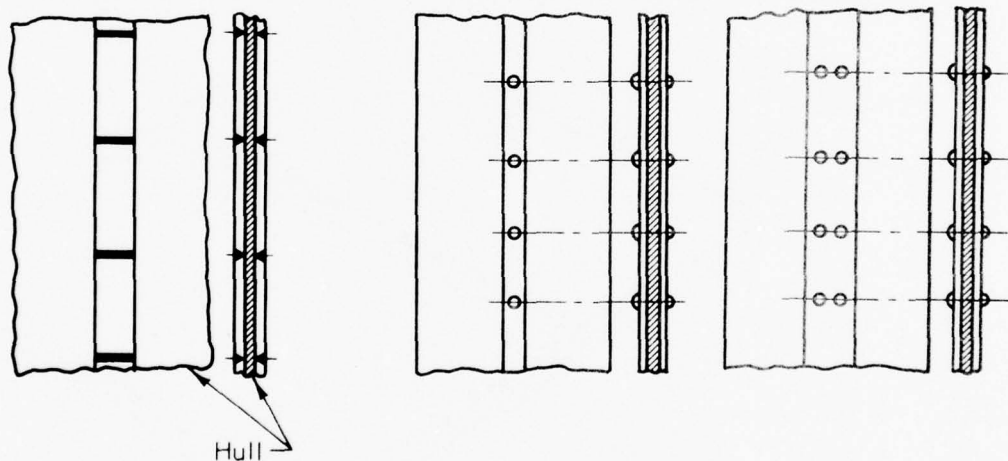
Welded Patch Type
