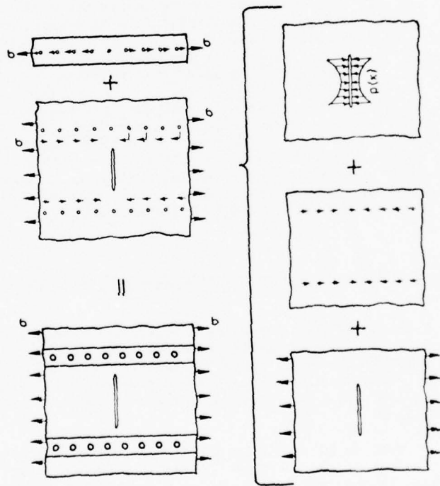
FIGURE 3.5.1. ANALYSIS OF STIFFENED PANEL
