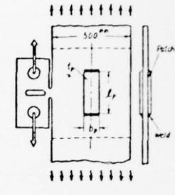
(a) Welded Patch Type
