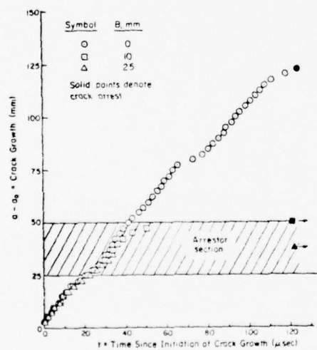
FIGURE 3.6.3.(a). CRACK PROPAGATION COMPUTATIONS FOR A DCB SPECIMEN WITH AN INTERMITTANTLY ATTACHED STIFFENER CRACK ARRESTER FOR K_q/K_{IC} = 2.0
