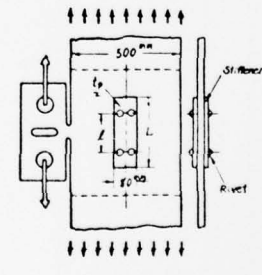
(c) Riveted Stiffener Type
