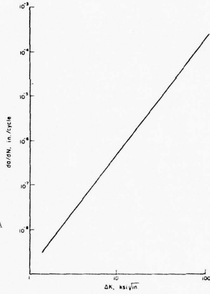
FIGURE 4.5.3. ASSUMED CRACK RATE PROPERTIES FOR CRACK-GROWTH CURVES IN FIGURE 4.5.2
