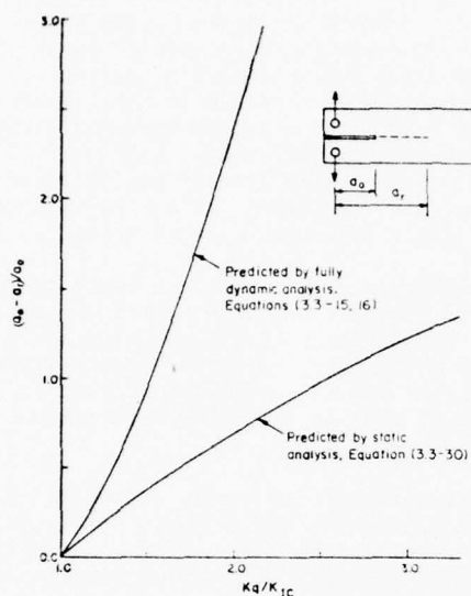
FIGURE 3.6.4. COMPARISON OF CRACK ARREST POINT IN A DCB TEST SPECIMEN WITH STATIC AND WITH FULLY DYNAMIC ANALYSIS
