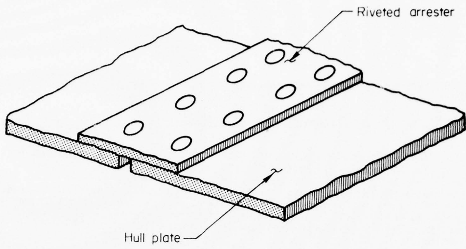
FIGURE 2.2.1. RIVETED SEAM TYPE OF CRACK ARRESTER
