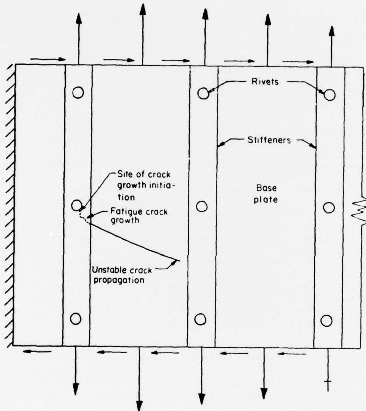
FIGURE 7.1.1. REINFORCED SHIP HULL
