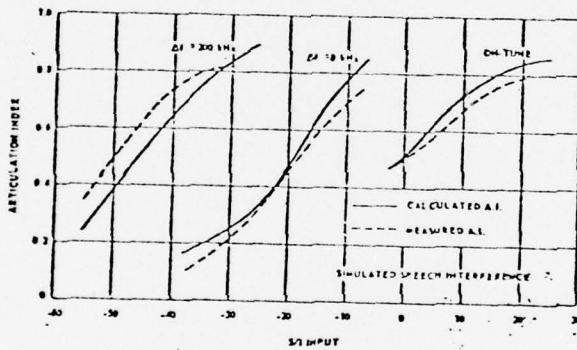
Performance Calculated From Nominal Receiver Characteristics
