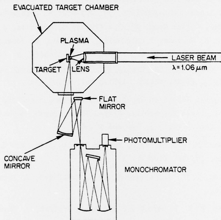
Fig. 1 — Experimental arrangement
