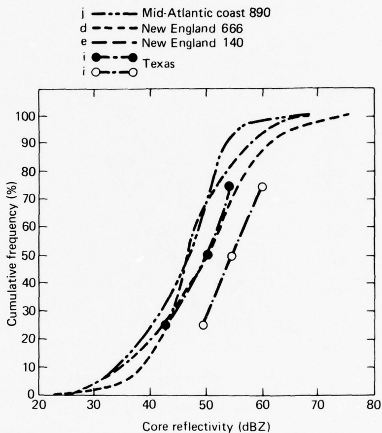
Fig. 21 Frequency Distributions of Core Reflectivity at 1.5-km Altitude for Various Locations. The Texas data with solid symbols were taken in 1959, open symbols in 1960.
