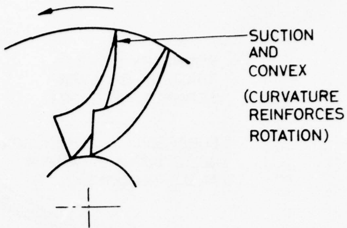
(a) RADIALLY BLADED IMPELLER
