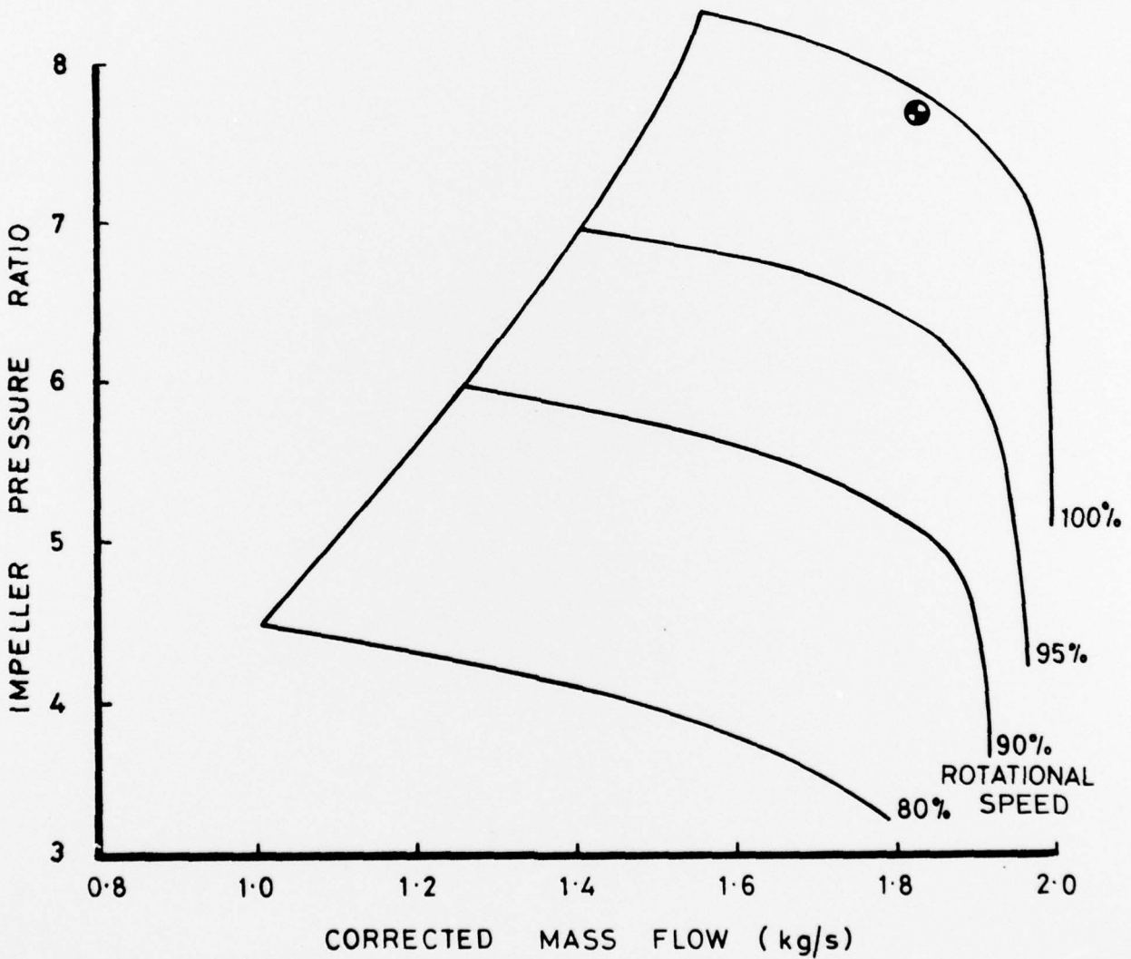
FIG. 41 COMPRESSOR 'B' ~ IMPELLER ALONE PERFORMANCE
