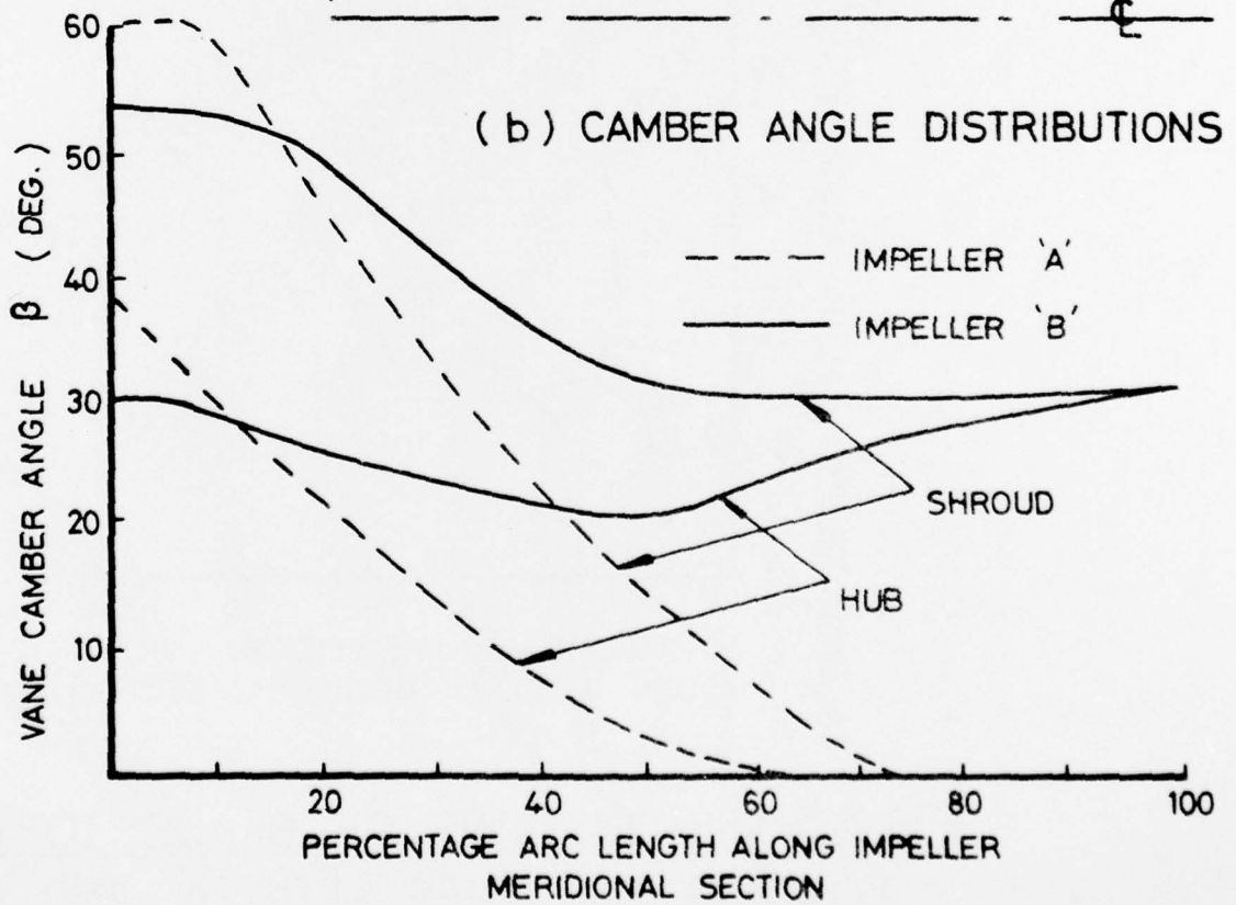
FIG.39. GEOMETRIC COMPARISON OF IMPELLER 'A' AND IMPELLER 'B'
