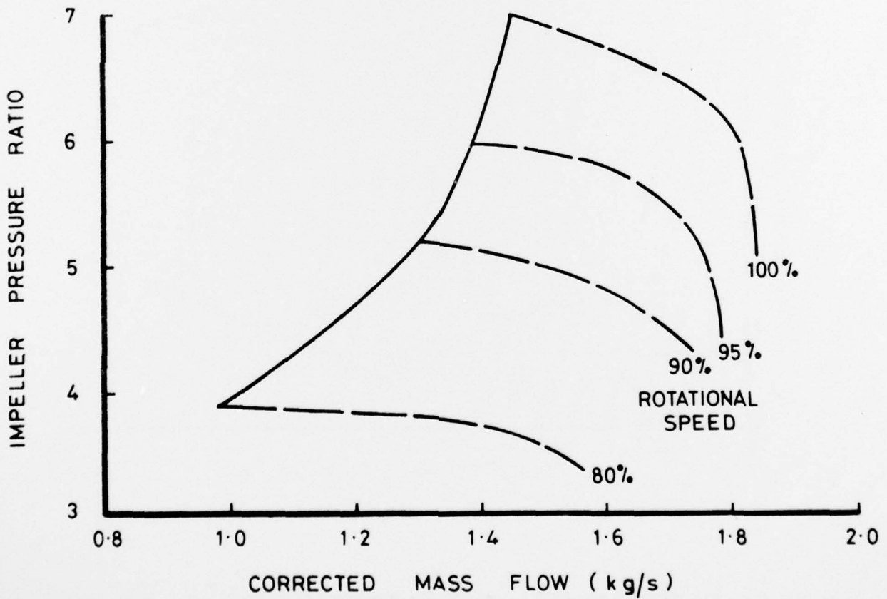
FIG. 38 · COMPRESSOR 'A' ~ IMPELLER ALONE PERFORMANCE
