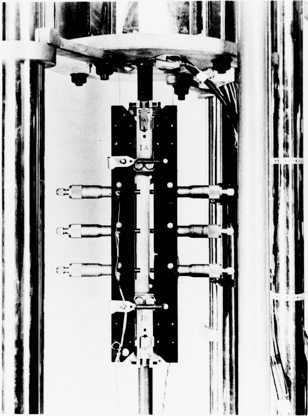
Fig.8 Width alignment
