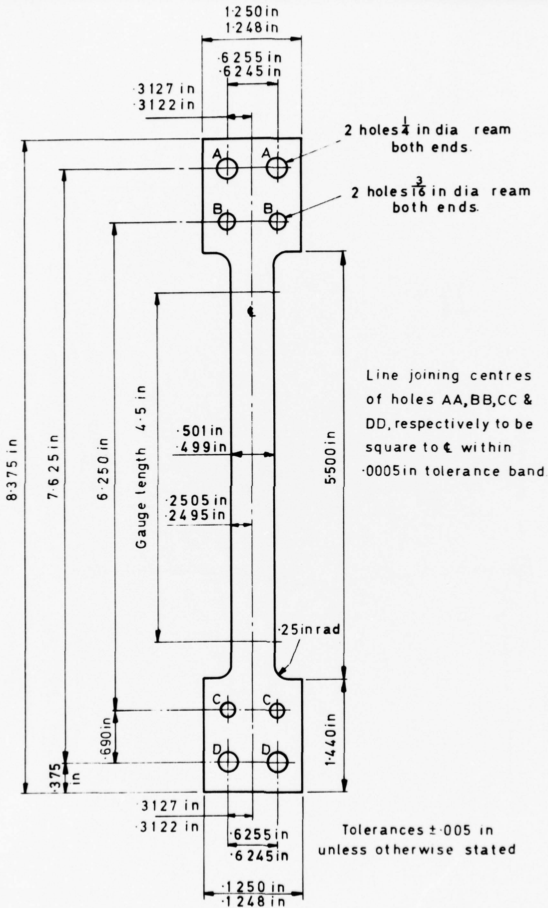
Fig.2 Test specimen of BNF design.
