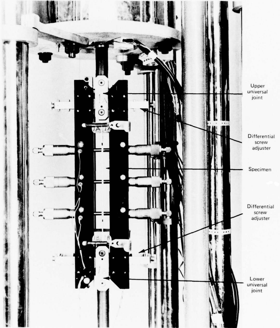
Fig.7 Thickness alignment
