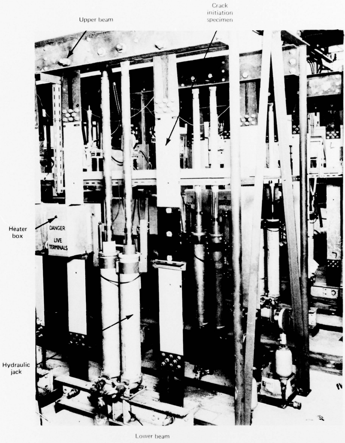
Fig.3 General arrangement of specimens and rig
