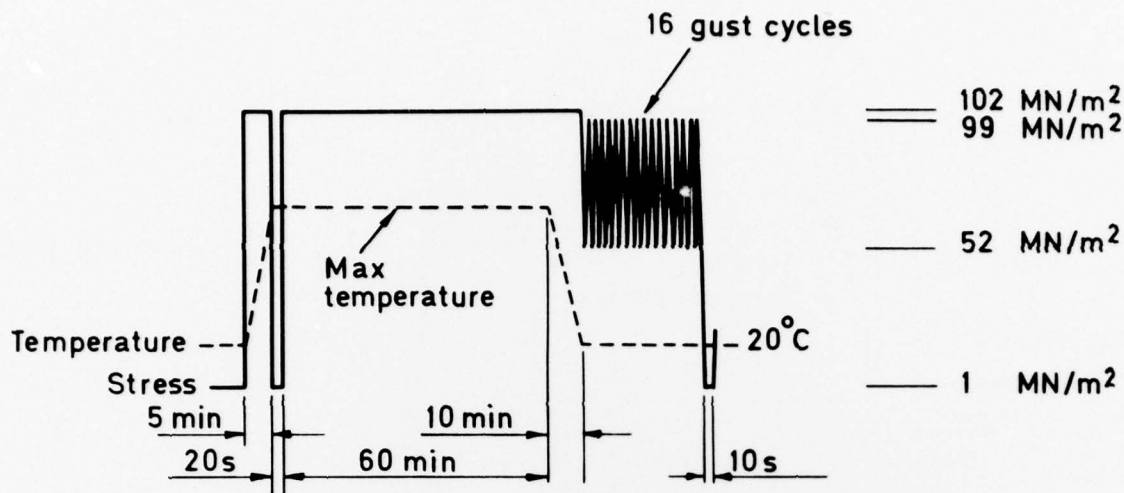
a Intermittent creep flight cycle
