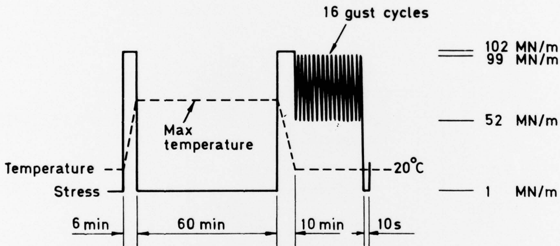
b Intermittent heating flight cycle
