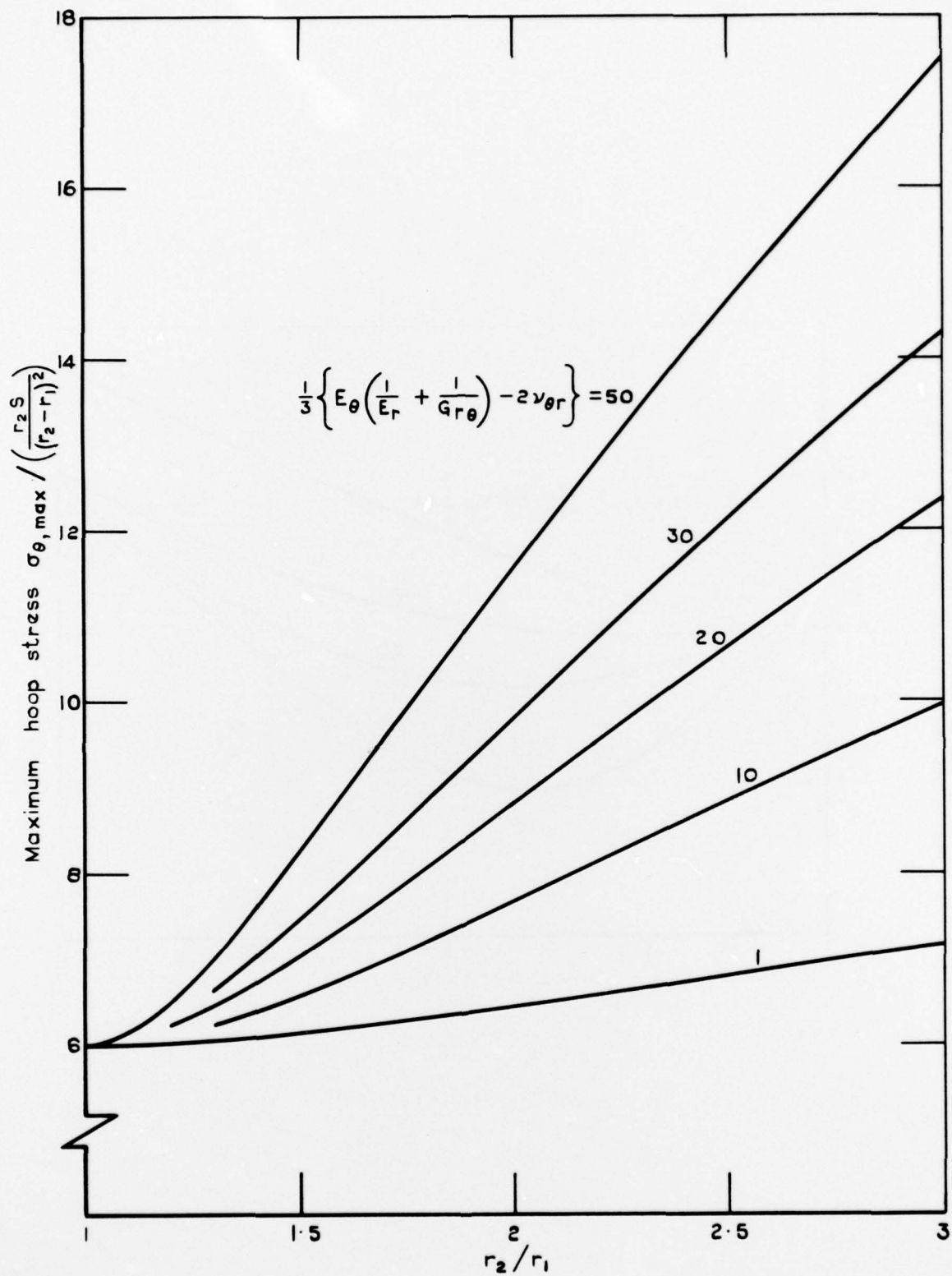
FIG. 13. Maximum hoop stress due to shear force.
