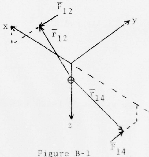
Geometry of Thrusters
