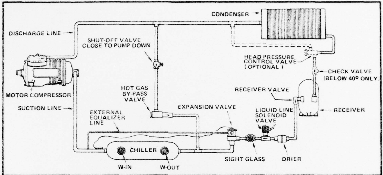
Figure 6. Refrigeration system layout of the heat pump
