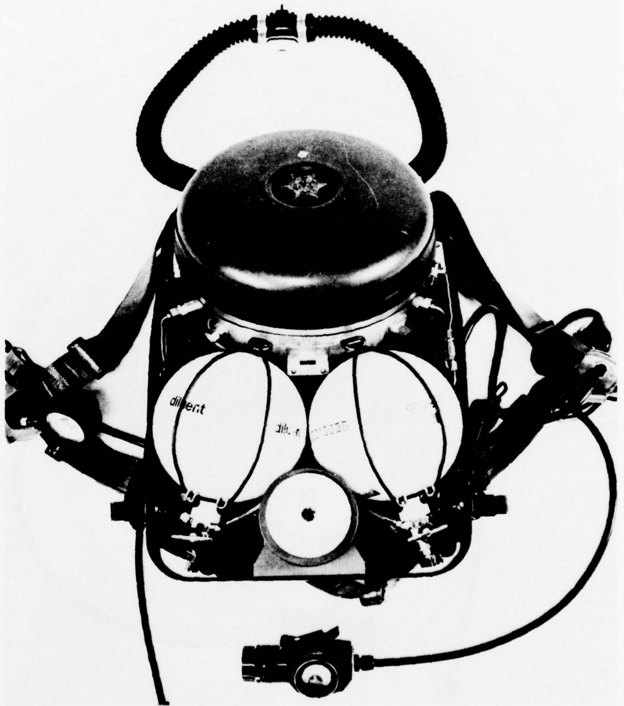
FIGURE 6. INTERNAL VIEW OF SLSS MK 1 (BOTTLES INSTALLED) XVI
