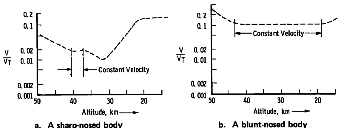
Figure 4. A schematic for shape influences on altitude histories; wake velocity measurements at a fixed distance from the nose.
