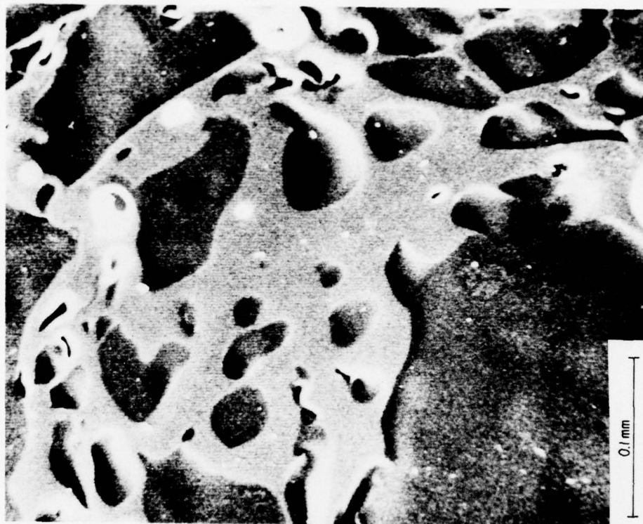
Figure 19. a) Scanning electron micrograph of an external part of char shown in Figures 17 and 18; b) portion of a) at higher magnification.
