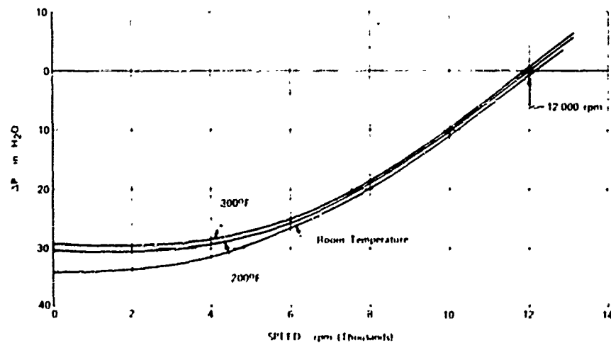
FIGURE 2.80 AVAILABLE DATA: PROPORTIONAL SHAFT RATE SENSOR - HONEYWELL
