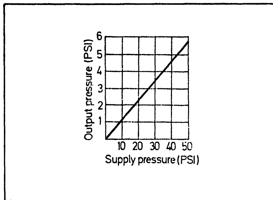
FIGURE 2.46 AVAILABLE DATA-INTERRUPTIBLE JET SENSOR-FESTO
