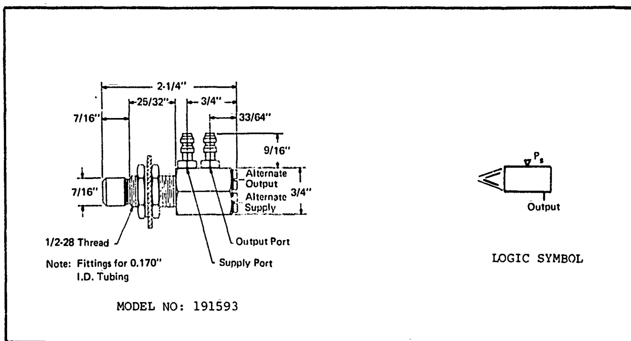
FIGURE 2.12 CONE JET SENSOR-CORNING
