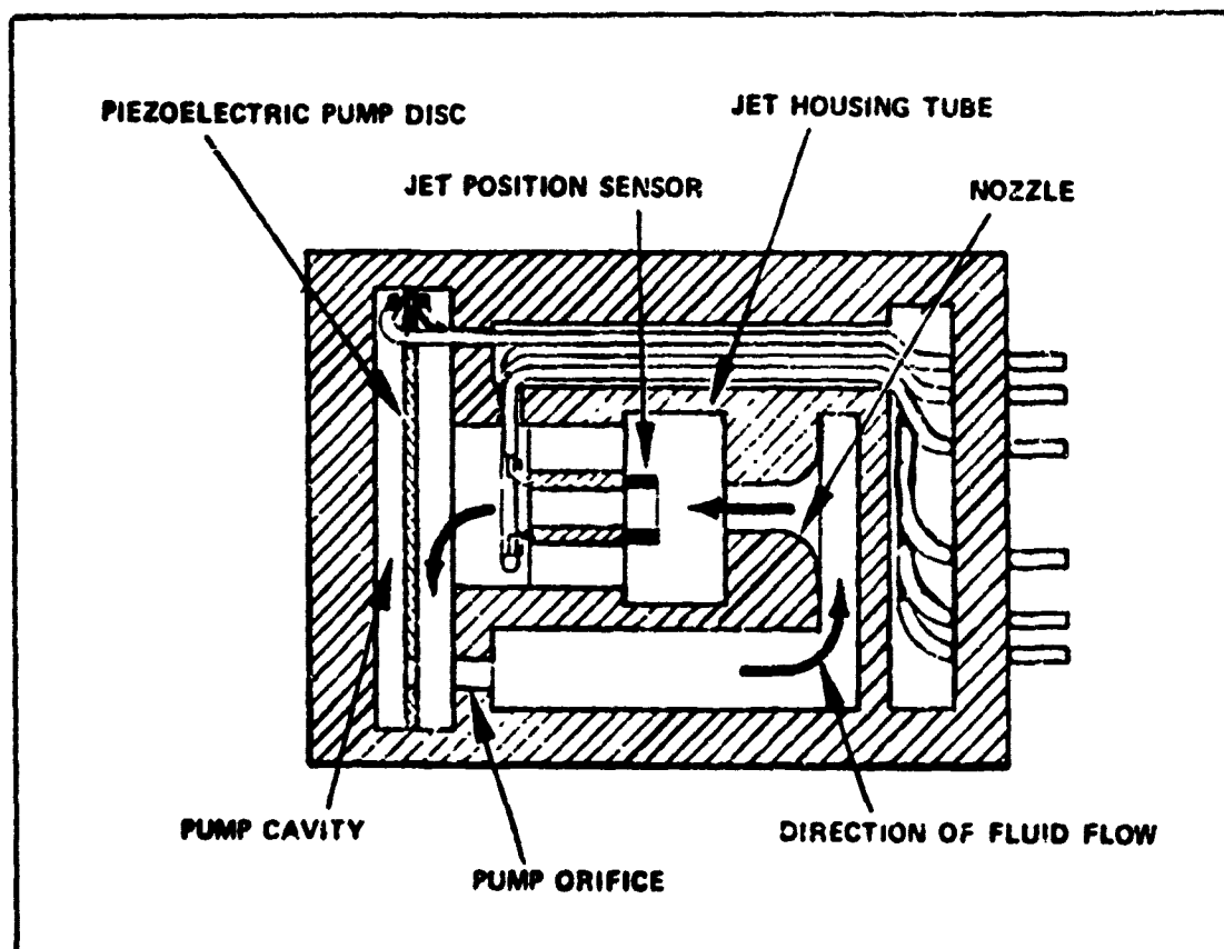
FIGURE 2.83 HYBRID RATE SENSOR
