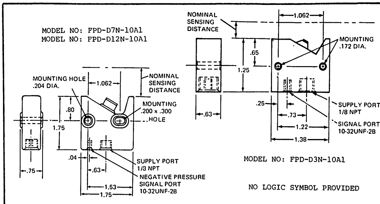
FIGURE 2.34 ANNULAR NOZZLE-PROXIMITY SENSOR-BROWN & SHARPE
