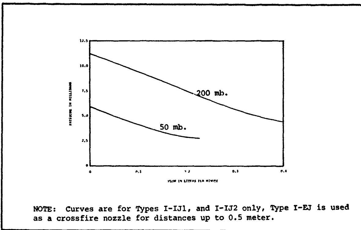
FIGURE 2.41 AVAILABLE DATA-INTERRUPTIBLE JET SENSOR-BRITISH FLUIDICS AND CONTROLS
