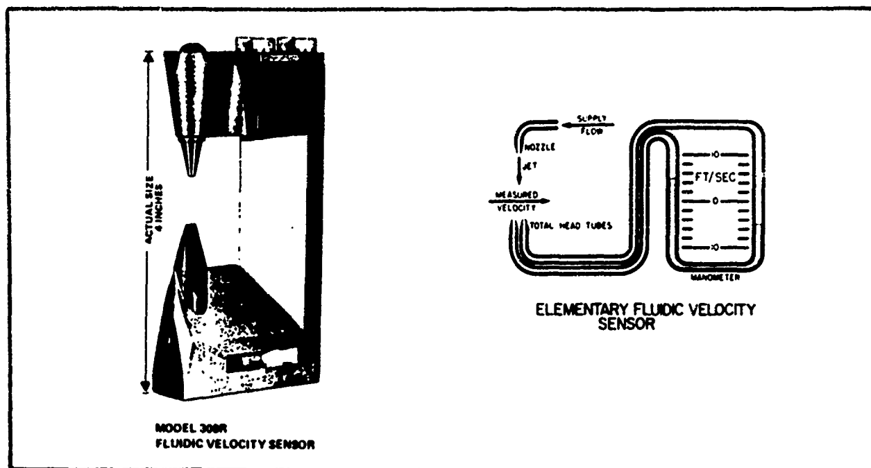
FIGURE 2.121 JET DEFLECTION VELOCITY SENSOR-FLUIDYNAMIC DEVICES LTD.
