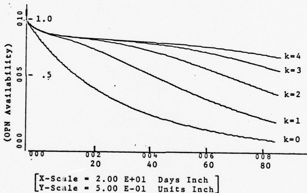
Figure 4. Operational Availability, A_k(t) .
