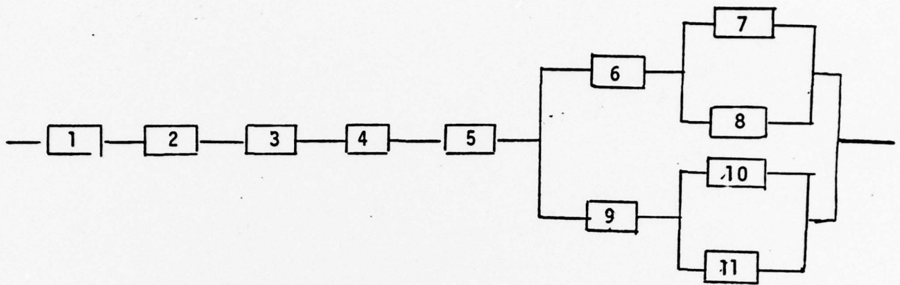
Figure 7. System Reliability Block Diagram.
