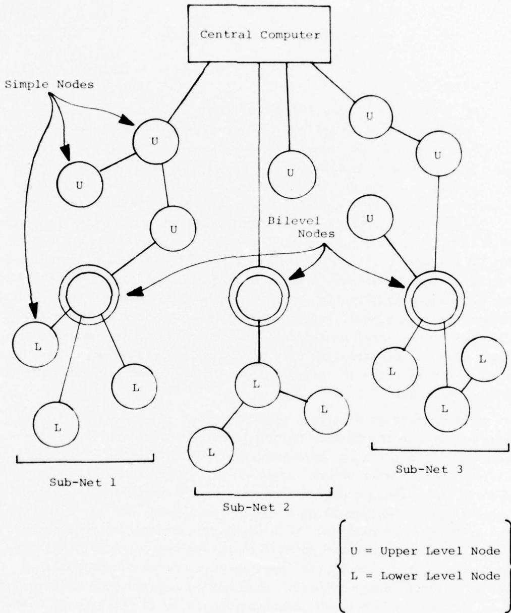
Figure 4.1 The Bilevel Network Concept.
