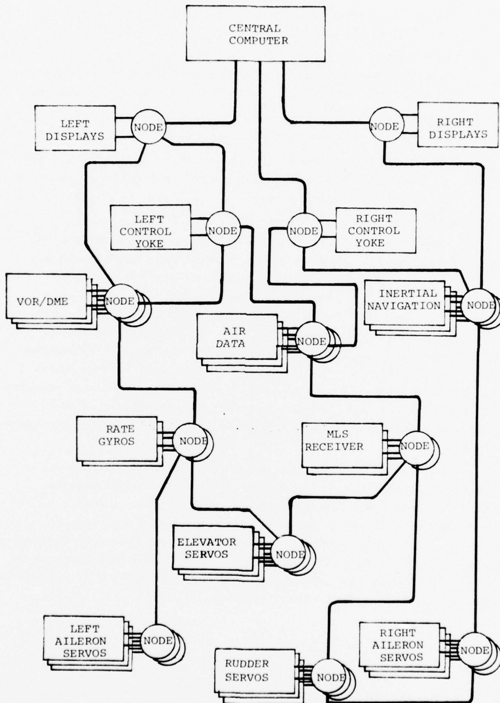
Figure 2.3 Hypothetical Distribution of Aircraft Node Locations.
