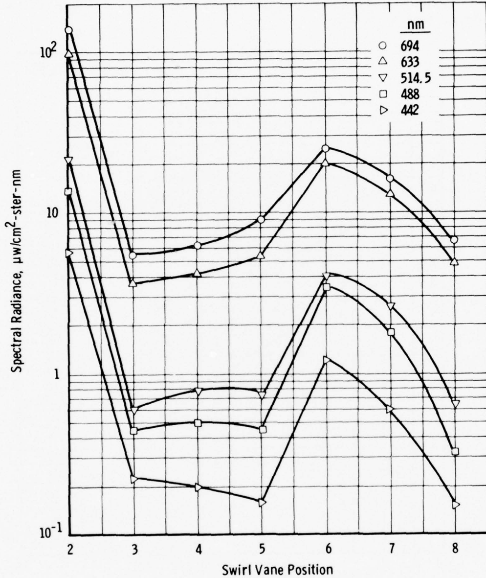
Figure 8. Spectral radiance as a function of vane position (fuel oil at position 1).
