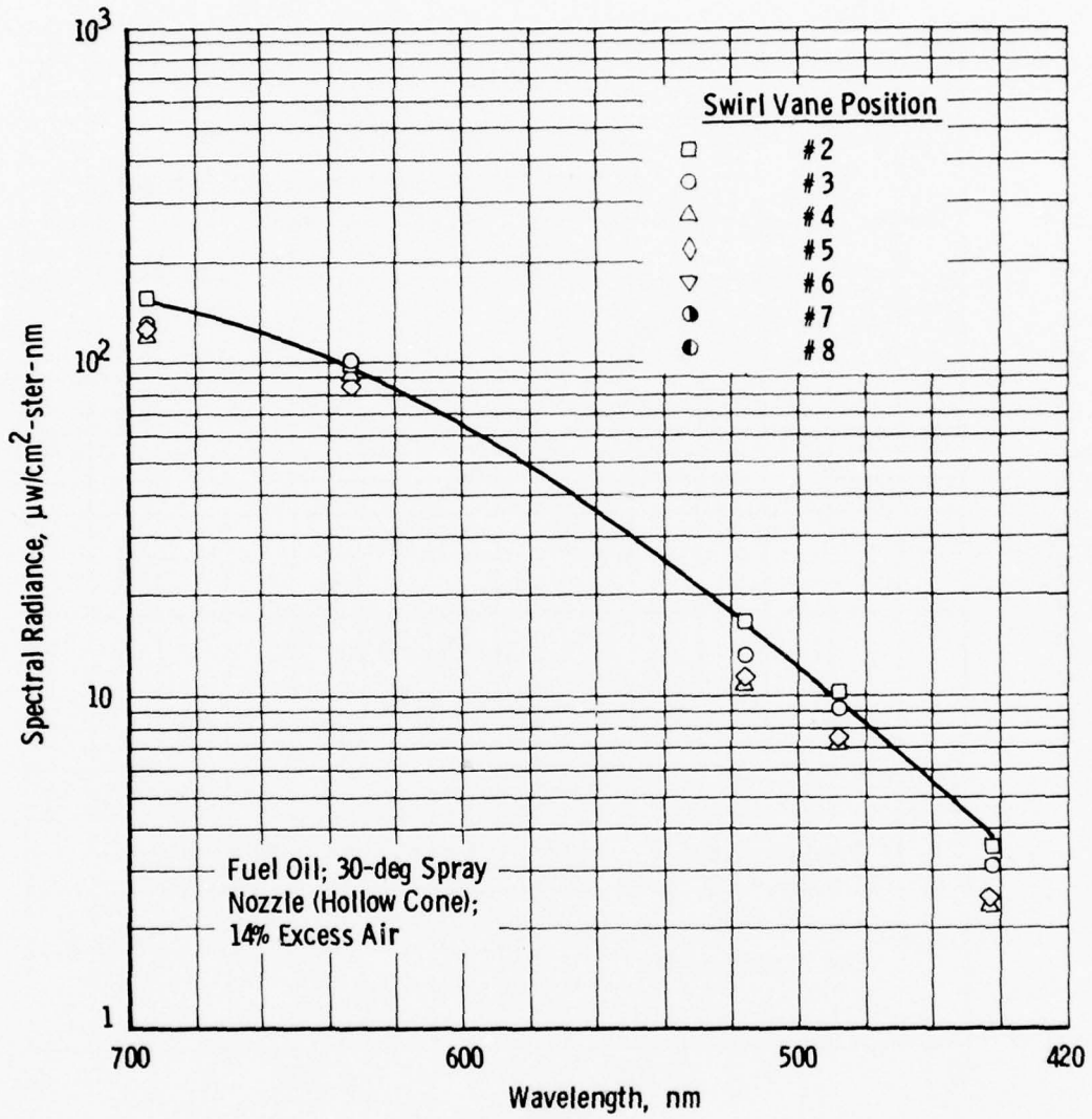
Figure 9. Spectral radiance as a function of wavelength (fuel oil at position IV).
