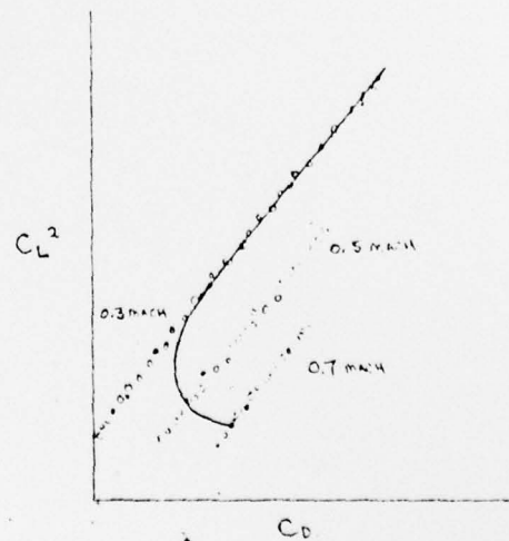
Figure 3. Windup Turns
