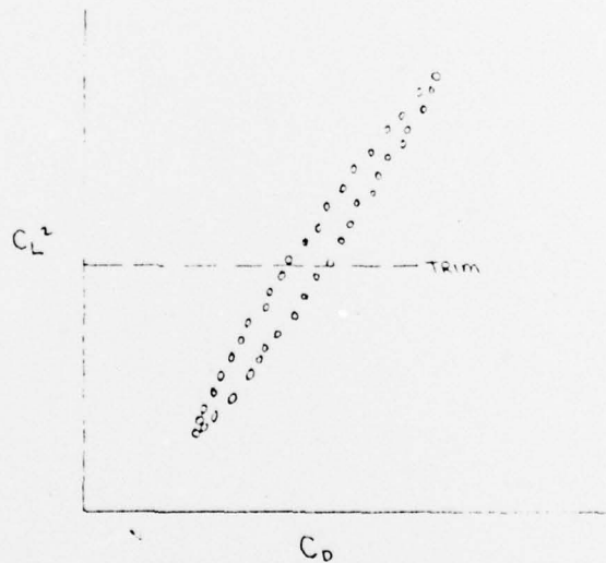
Figure 6. Roller Coaster with Response Error
