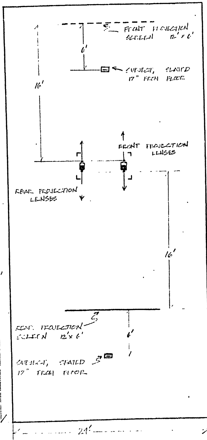
Figure III - Laboratory Layout
