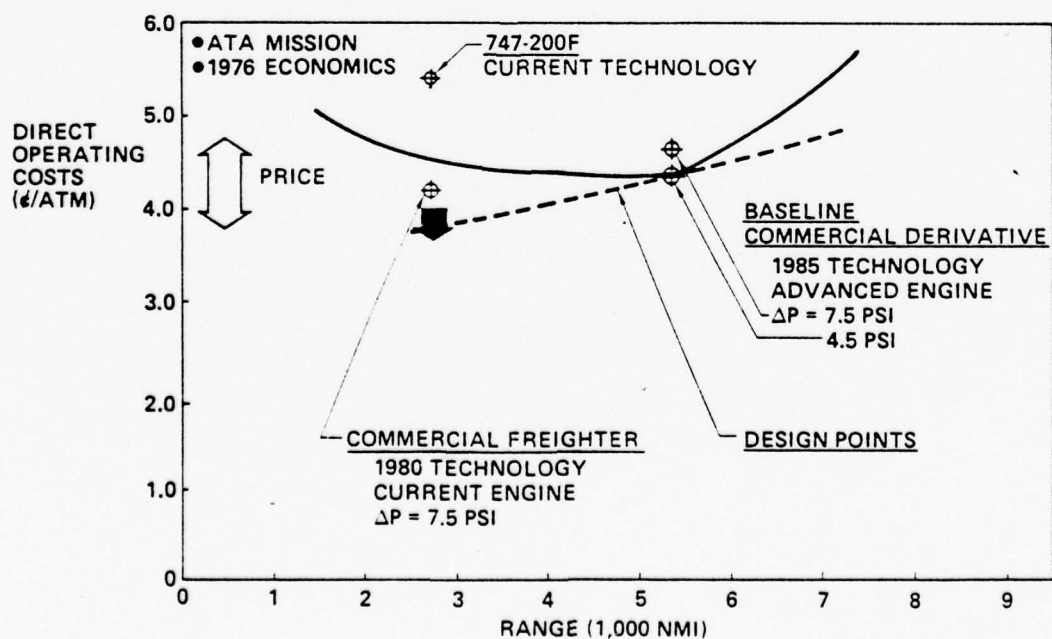
Figure 6-7 Commercial Commonality Direct Operating Costs
