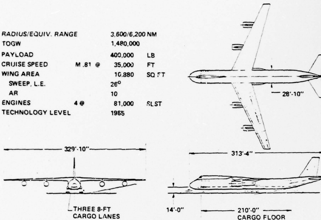
Figure 3.26. Model 1044-014 IADS Airplane Three Cargo Lanes
