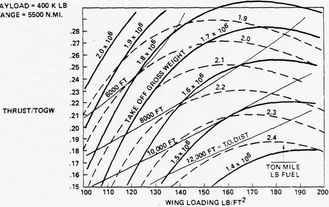
Figure 2-9, Composite Design Chart Range Optimized
