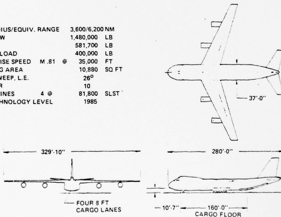
Figure 3.27. Model 1044-013 IADS Baseline Airplane Phase II — Four Cargo Lanes
