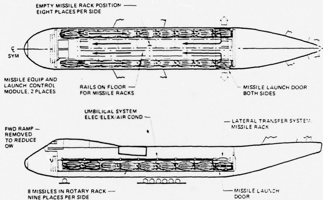
Figure 5-7. ALCM Carrier
