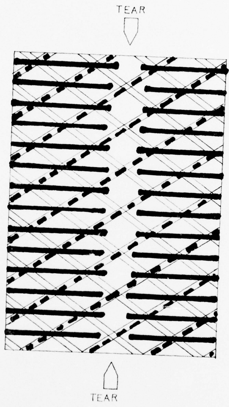
Figure 2. Triaxial Fabric
