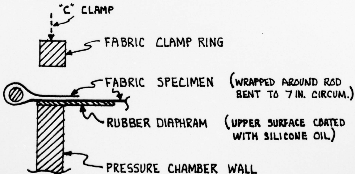
Figure B-2 Cross-Sectional View of Figure Clamp
