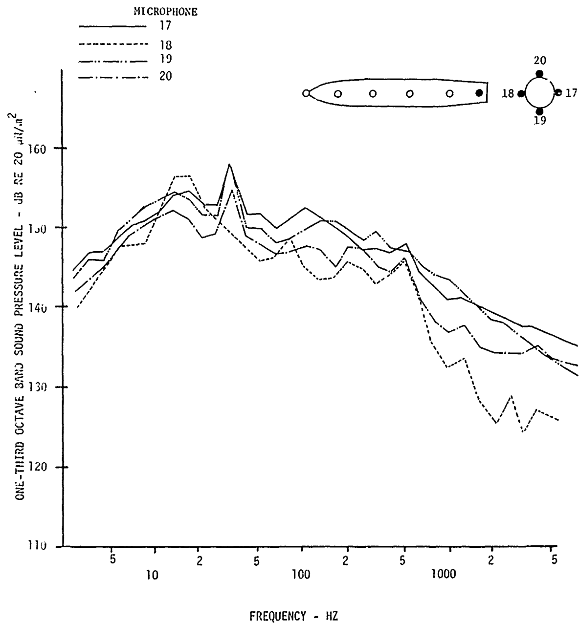
FIGURE 15 CIRCUMFERENTIAL VARIATION AT STATION 154 OF ONE-THIRD OCTAVE BAND SPL SPECTRA FOR A MACH NUMBER OF 0.95 AND A 30,000 FOOT ALTITUDE
