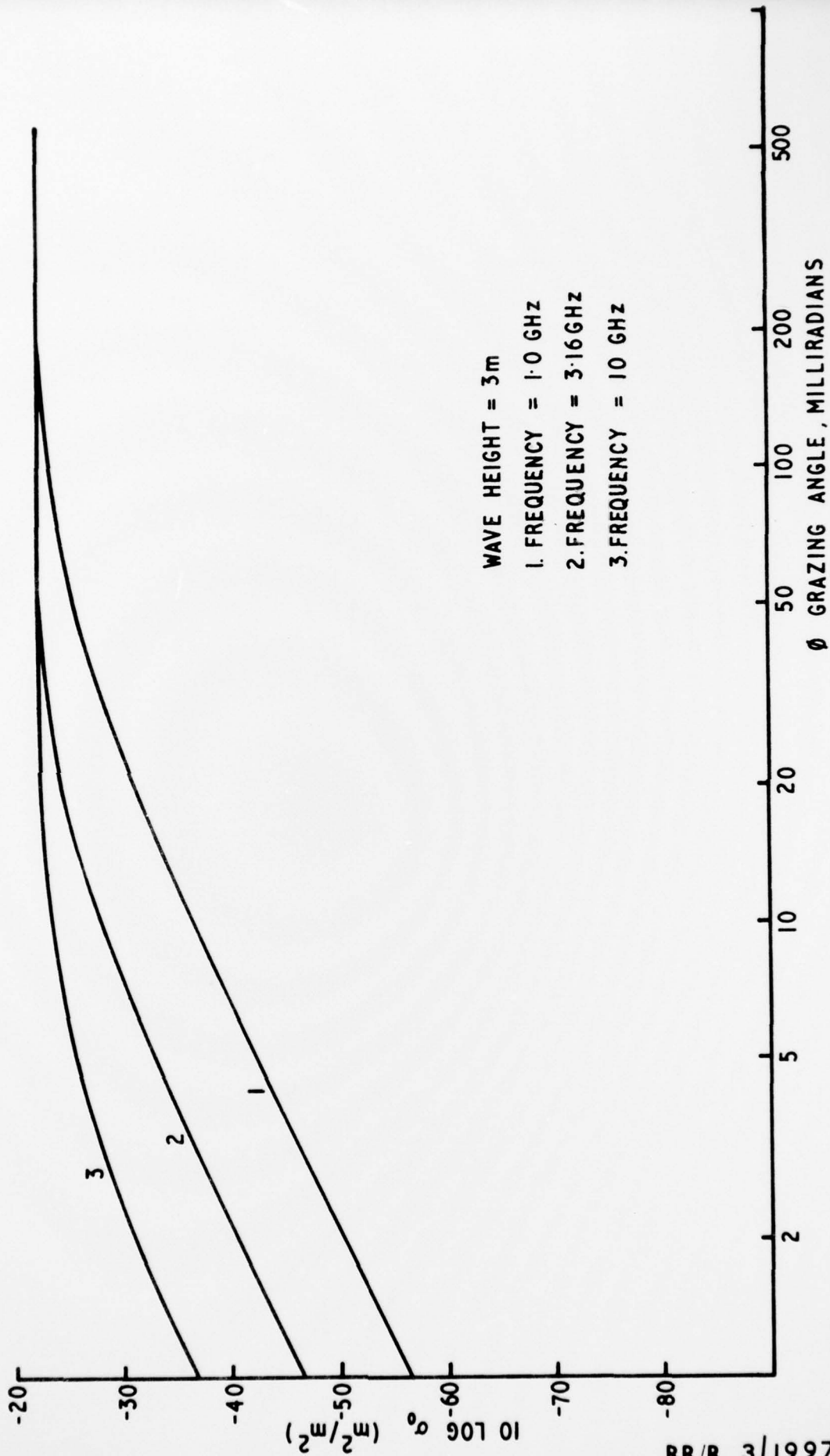
FIG. 12 SURFACE REFLECTIVITY (σ 0 ) OF THE SEA. VERTICAL POLARISATION
