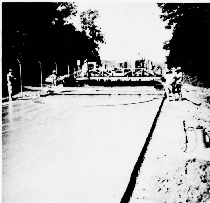
Figure A1. Slip-form paver placing 4-in.-thick pavement
