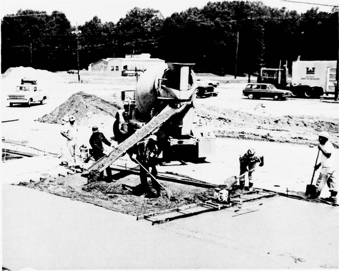
Figure A5. Double beam type vibratory screed
