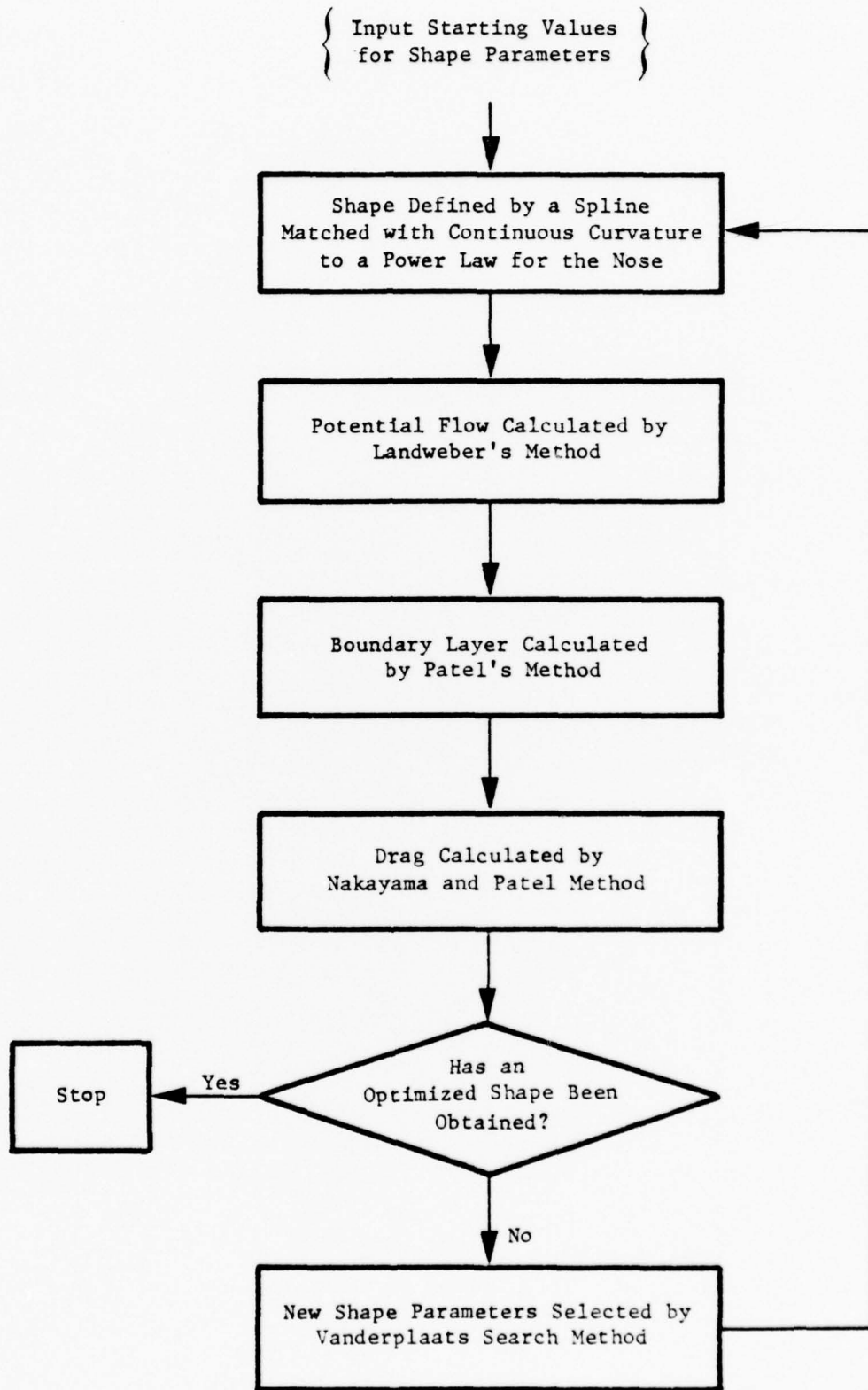
Figure 2 Flow Chart for Computer Program No. 2
