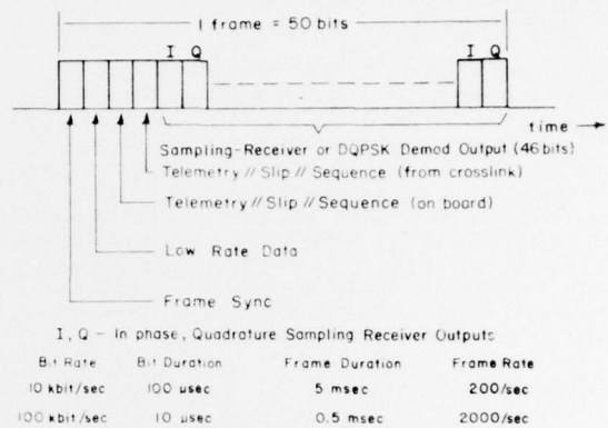
Figure 13. CROSSLINK DATA FORMAT
