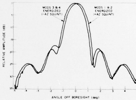
Figure 7. LOBED ANTENNA PATTERNS
