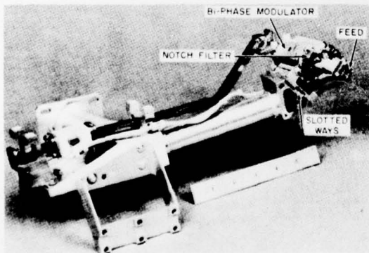
Figure 6. LOBING FEED ASSEMBLY
