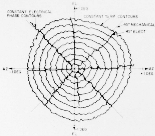
Figure 8. LOBING SENSITIVITY AND ORTHOGONALITY
