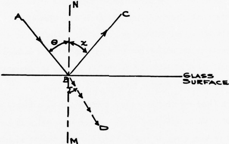
FIGURE 3.2 FIRST SURFACE REFLECTION (GLASS)
