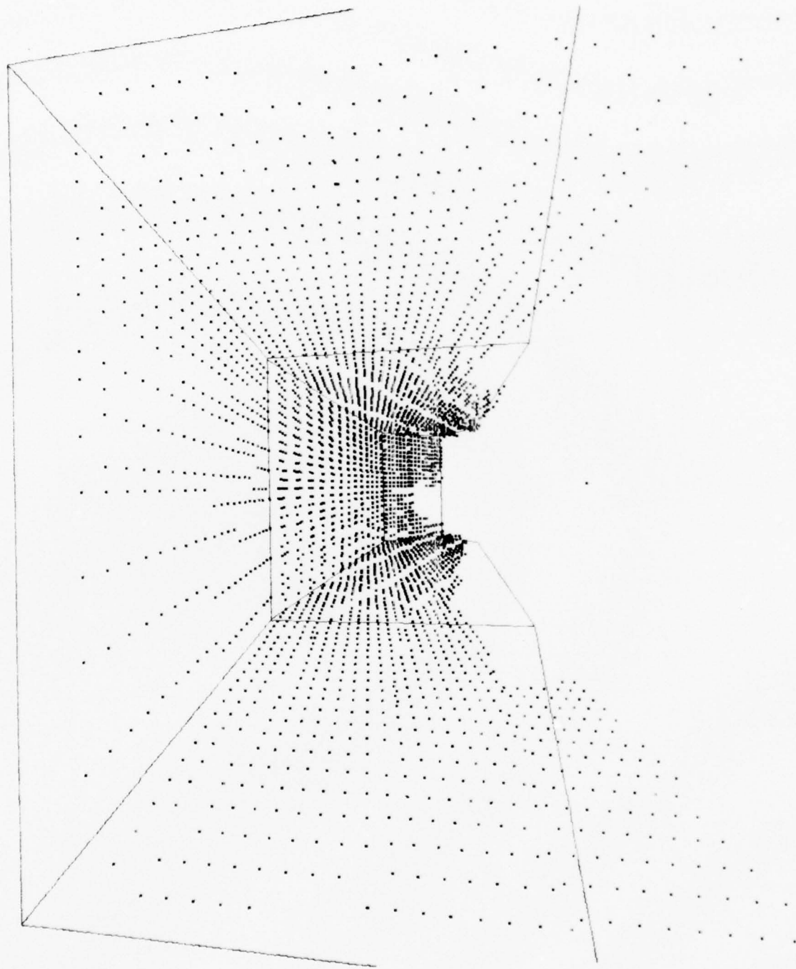
Figure 1A. Perspective view from pilot's position of all possible entry points for external light rays on right-hand side of FPC.
