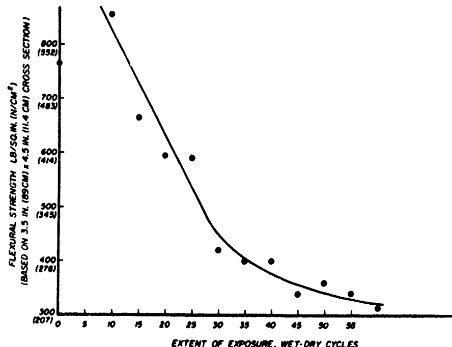
Figure 29. Loss of flexural strength of preflawed specimens at various degrees of exposure.
