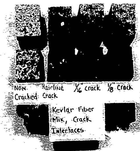
Figure 11. Kevlar specimen crack interfaces.
