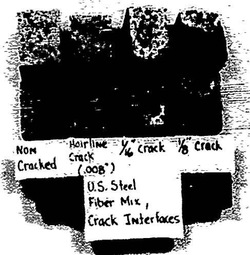
Figure 13. U. S. Steel specimen crack interfaces.
