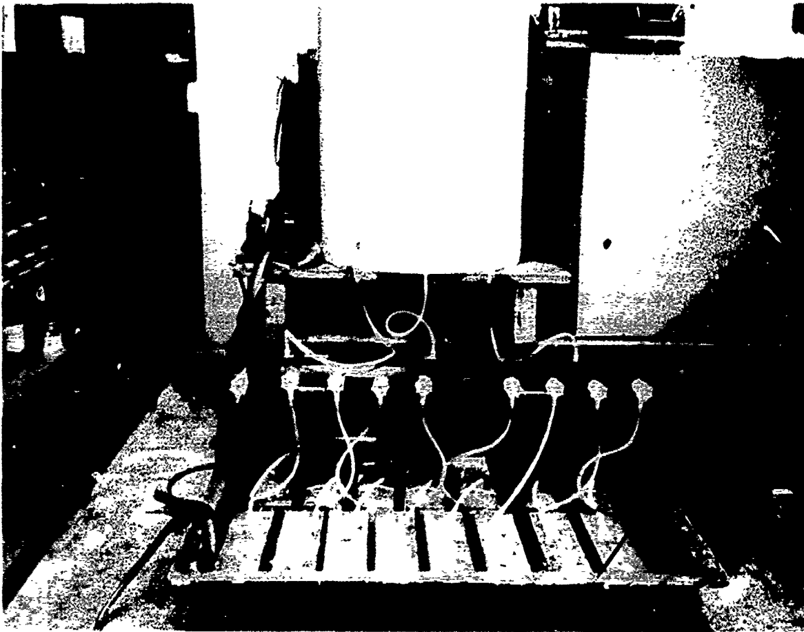
Figure 24. Wet-dry saltwater exposure apparatus.
