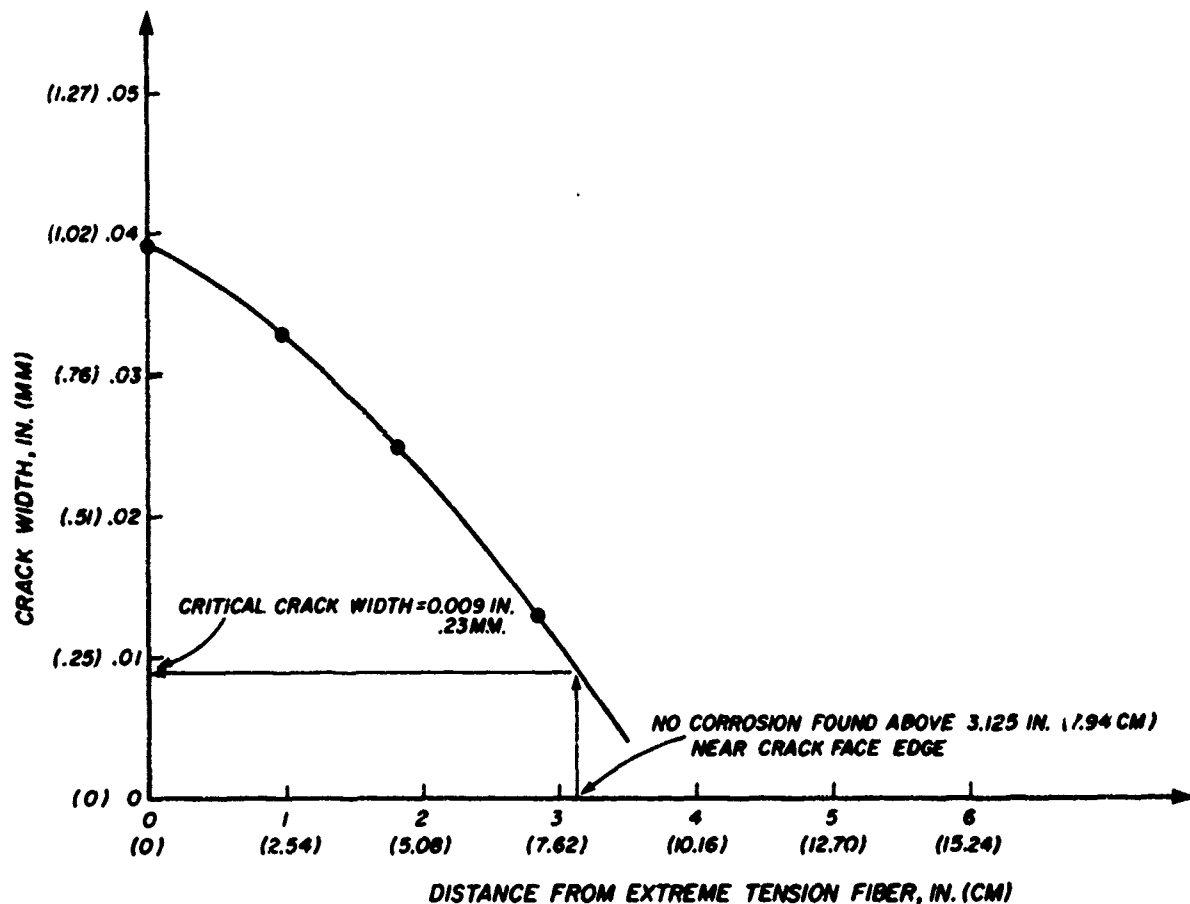
Figure 16. Typical crack width variation.
