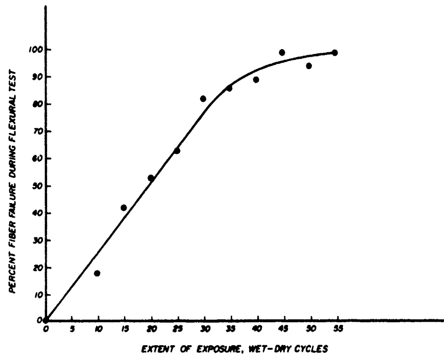
Figure 28. Loss of fiber integrity during flexural test for preflawed specimens of various degrees of exposure.
