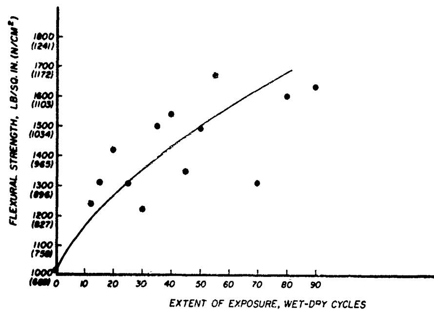
Figure 30. Strength development of unflawed specimens due to moist corrosive environment.
