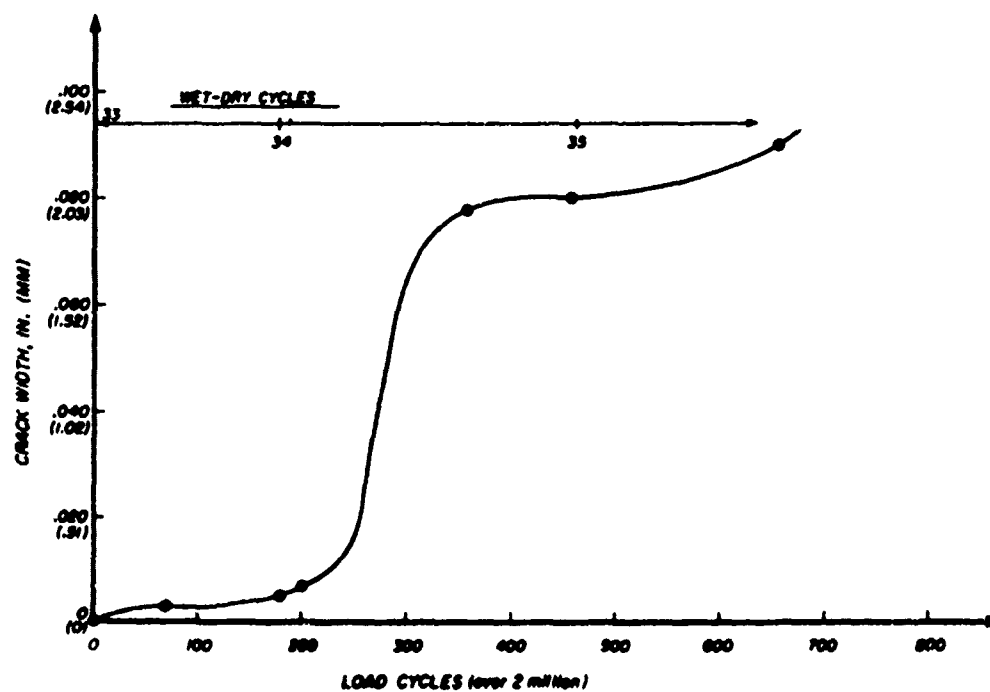
Figure 36. Load cycles vs. crack width for beam in corrosive environment.
