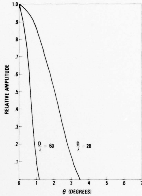
Fig. 15—Sensitivity vs angle from the axis of the transducer for a flat circular reflector
